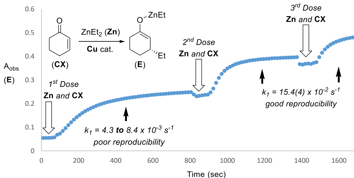
Figure 1. ReactIR observation of the 7/L A catalysed formation of enolate ( E ) via its 1145 \text{ cm}^{-1} band in a multiple dosing experiment. As each reaction completes fresh \text{ZnEt}_2 ( Zn ) and cyclohex-2-en-1-one ( CX ) is added and catalysis restarts. First dose experiments show poor reproducibility (see Figure S6, Supporting Information), but the 2 nd and 3 rd dose derived first order rate constants show good reproducibility when allowing for the dilution occurring in the reaction from dose 2 to 3.
