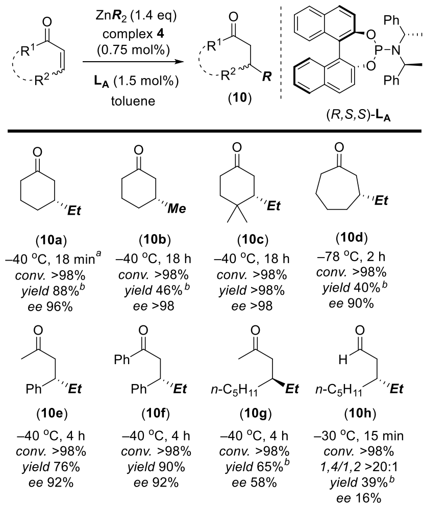
Scheme 3. Benchmarking enone studies demonstrating the high activity of the ( 7 )/ \text{L}_A catalyst. a Full conversion is attained within 2 h at −80 °C. b The lower isolated yields reflect isolation issues for volatile products 10 associated with toluene solvent removal, using \text{Et}_2\text{O} results in yields in line with conversion. Quantification against internal standards indicated excellent conversion and mass balance.
