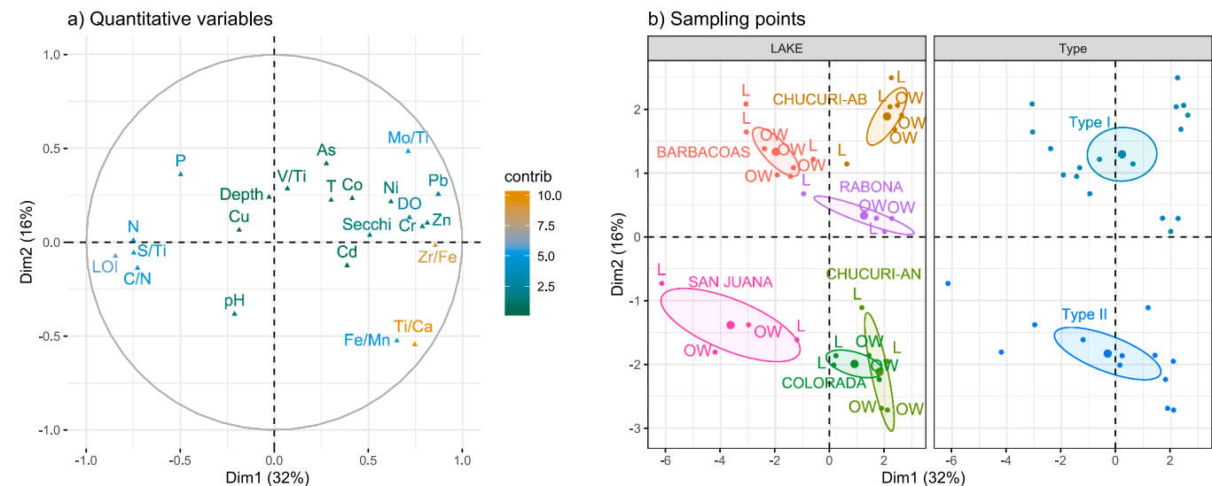
Fig. 2. Multiple Factor Analysis (MFA) plots illustrating: (a) the variations of OM (LOI and C/N), redox conditions (Fe/Mn, S/Ti, V/Ti and Mo/Ti), flooding (Zr/Fe ratio), erosion (Ti/Ca ratio), heavy metals (Mn, Cr, Co, Ni, Cu, Zn, As, Cd, and Pb), nutrients (P and N), and water chemical parameters (DO, surface temperature [T], pH, Secchi depth, and water depth) in the surface-sediments of the lakes. The pale brown background represents conditions high in OM, while the blue background indicates environments dominated by heavy metals, erosion, flooding, and reductive conditions; (b) The sampling locations within each lake are categorised by hydrological connectivity type: L = littoral; OW= open water.
