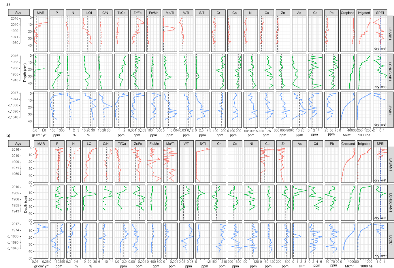
Fig. 3. Stratigraphic plot showing the long-term variation in biogeochemical elemental concentrations and mean values (dash vertical lines) in (a) connected lakes (Type I); and (b) more isolated lakes (Type II). Wet and dry interannual periods as indicated by SPEI are also shown by a blue vertical line.
