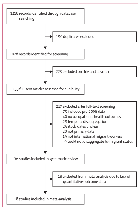
Figure 1: Study selection
