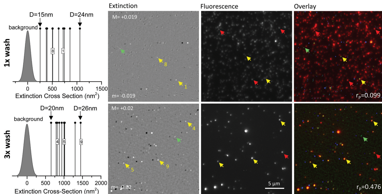
Fig. 6 20 nm AuNP-PC-Ab(A647) imaged by correlative wide-field fluorescence and extinction microscopy. The AuNP solution was washed once (top) or 3 times (bottom) to reduce the presence of unbound antibodies. AuNPs were deposited on glass and imaged in air. Extinction cross-sections of ten representative single particles in the FOV are indicated on the left panels, with corresponding particle diameter ranges, above the detection limit (background histogram, see text). Extinction contrast images are shown on grey scale from m (black) to M (white), as indicated, with yellow arrows pointing to selected single AuNPs for which the cross-section was quantified, as labelled (images shown are 30% of the FOV). Fluorescence images of the same area are shown on a grey scale from 0.03F_m to 0.39F_m (top) and from 0.03F_m to 0.22F_m (bottom), with F_m being the maximum amplitude in the FOV. Overlay: fluorescence (red), extinction maxima (green) extinction minima (blue). In the overlay, amplitudes are re-scaled to maximize colour overlap. Green arrows indicate AuNPs visible only in extinction. Red arrows indicate unbound fluorophores. The cross-correlation (Pearson's) coefficient r_p is given.
