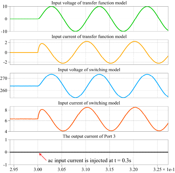
(d) Asymmetrical power flow: d_{21} = 0.1 , d_{31} = 0.05 with 100 Hz ac input current
