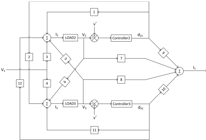
Fig. 5. The block scheme of TAB converter
