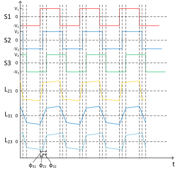
Fig. 4. The operating waveforms of TAB converter
