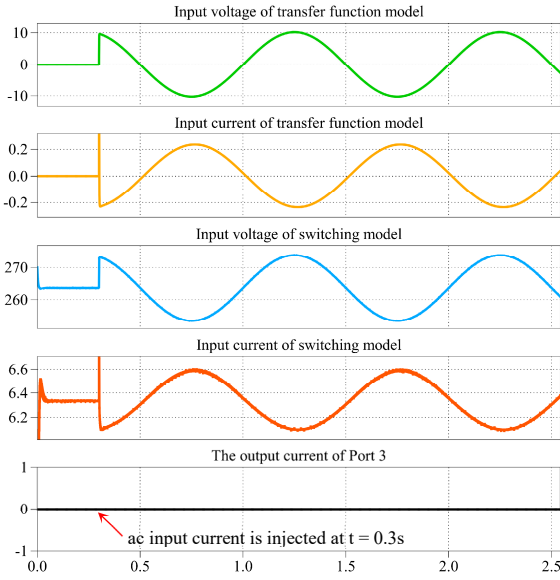
(c) Asymmetrical power flow: d_{21} = 0.1 , d_{31} = 0.05 with 1 Hz ac input current
