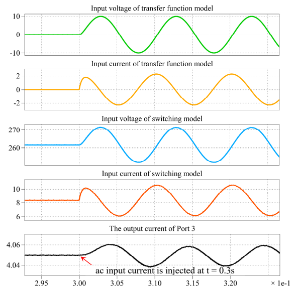
(b) Symmetrical power flow: d_{21} = d_{31} = 0.1 with 100 Hz ac input current
