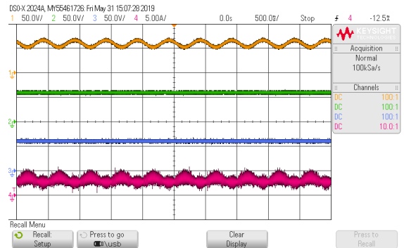
(a) Symmetrical power flow: 2 Hz ac component at input port
