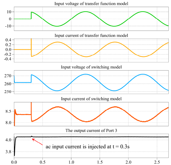
(a) Symmetrical power flow: d_{21} = d_{31} = 0.1 with 1 Hz ac input current
