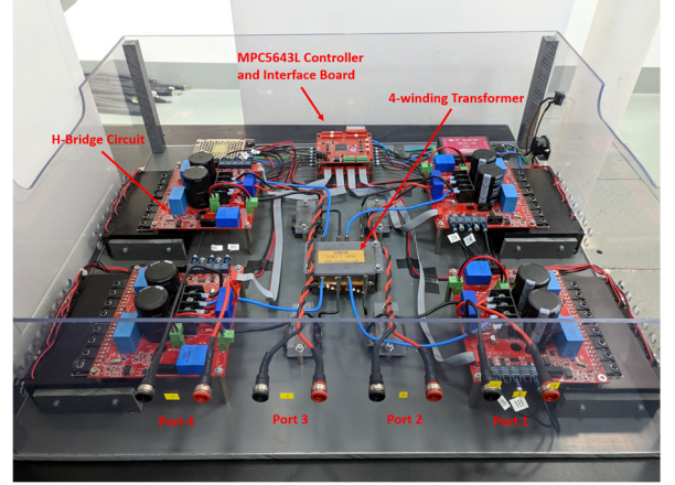
Fig. 8. Experimental prototype of TAB converter
