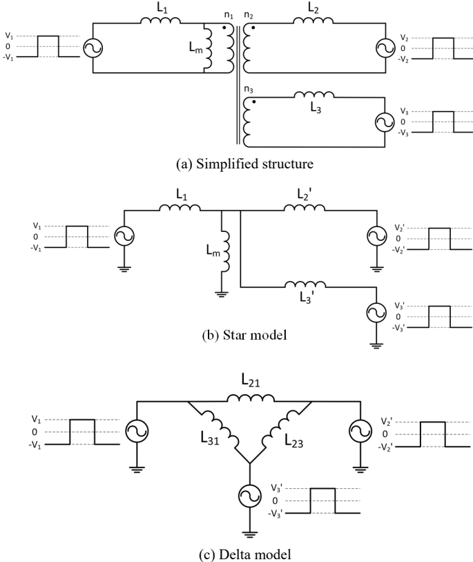
Fig. 3. The transformer model of TAB converter
