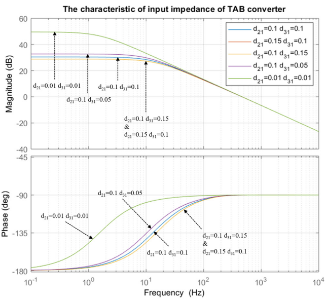
Fig. 6. The characteristic of input impedance of TAB converter
