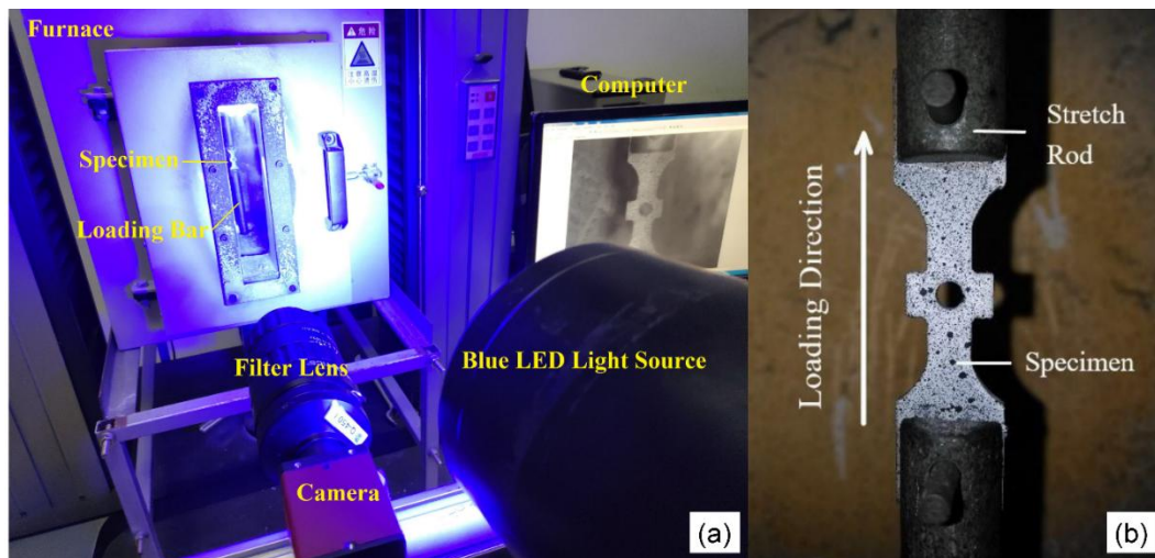
Fig. 3. (a) The experimental setup showing the digital camera used for the DIC measurements, a high temperature furnace, a narrow band pass filter lens of 441 \text{ nm} \pm 10 \text{ nm} bandwidth and a monochromatic light source with the wavelength of 440 \text{ nm} \pm 20 \text{ nm} . (b) The test specimen sprayed with a black/white speckle.
