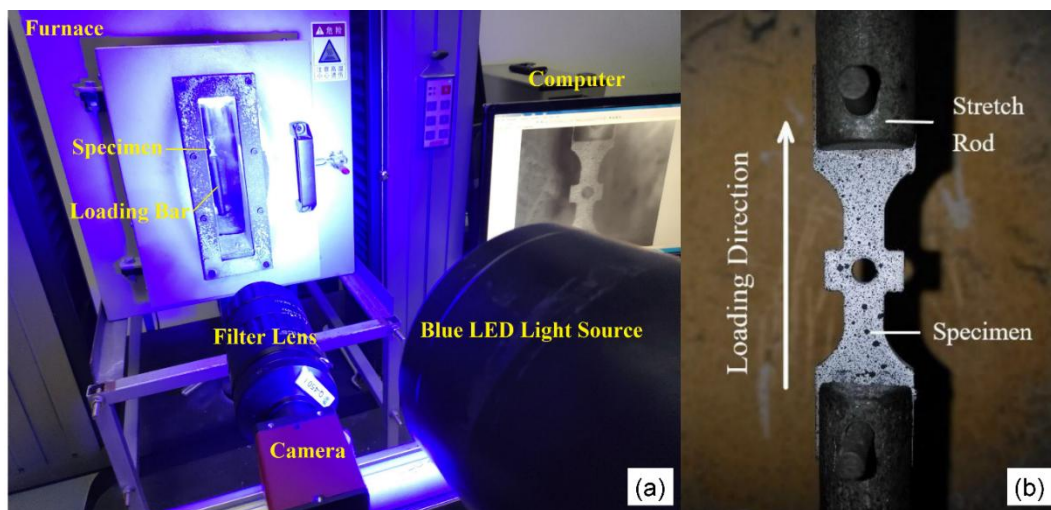
Fig. 3. (a) The experimental setup showing the digital camera used for the DIC measurements, a high temperature furnace, a narrow band pass filter lens of 441 \text{ nm} \pm 10 \text{ nm} bandwidth and a monochromatic light source with the wavelength of 440 \text{ nm} \pm 20 \text{ nm} . (b) The test specimen sprayed with a black/white speckle.
