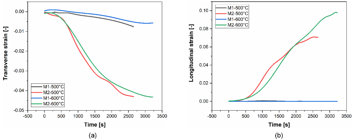
Fig. 9. (a) True transverse strain curves, and (b) true longitudinal strain curves with respect to the test time at M_1 and M_2 .
