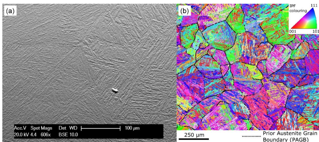
Fig. 1. (a) Backscattered electron image and (b) an EBSD orientation map of the as received FV566 material.
