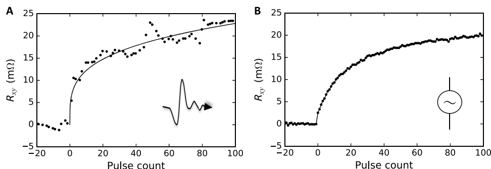
Fig. 4. Effects of individual picosecond and microsecond pulses. (A) The multilevel memory signal as a function of the number of applied picosecond pulses. The writing current density in the 2- \mu\text{m} -size CuMnAs/GaAs bit cell recalculated from the applied terahertz field amplitude is 2.9 \times 10^9 \text{ A cm}^{-2} . (B) Same as (A) for the microsecond pulses and an applied writing current density of 3 \times 10^7 \text{ A cm}^{-2} in the 3.5- \mu\text{m} -size CuMnAs/GaAs cell.
