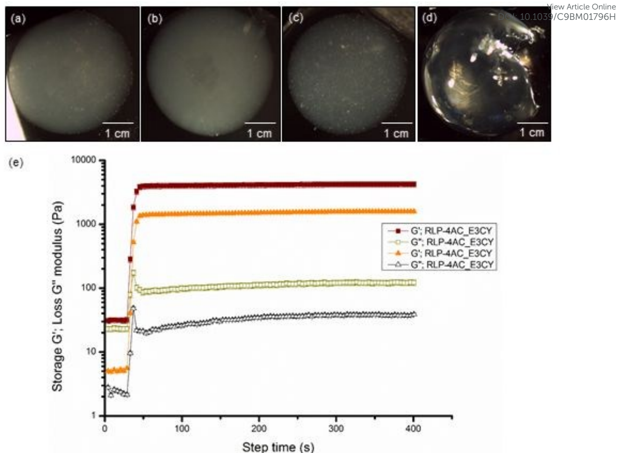
Figure 2. Optical image of hydrogels prepared with (a) thiol-ene photoclicked RLP-4AC (20 wt %)_ E3CY (1 wt % ), (b) RLP-4AC (20 wt %)_ E3CY (2 wt %), (c) photopolymerized RLP-4AC (10 wt %) and (d) E3CY- Ca 2+ (1 wt %). [Scale bar: 1 cm]. (e) Time sweep rheographs showing evolution of G' and G'' , confirming in situ hydrogel formation with 2 wt % E3CY .
