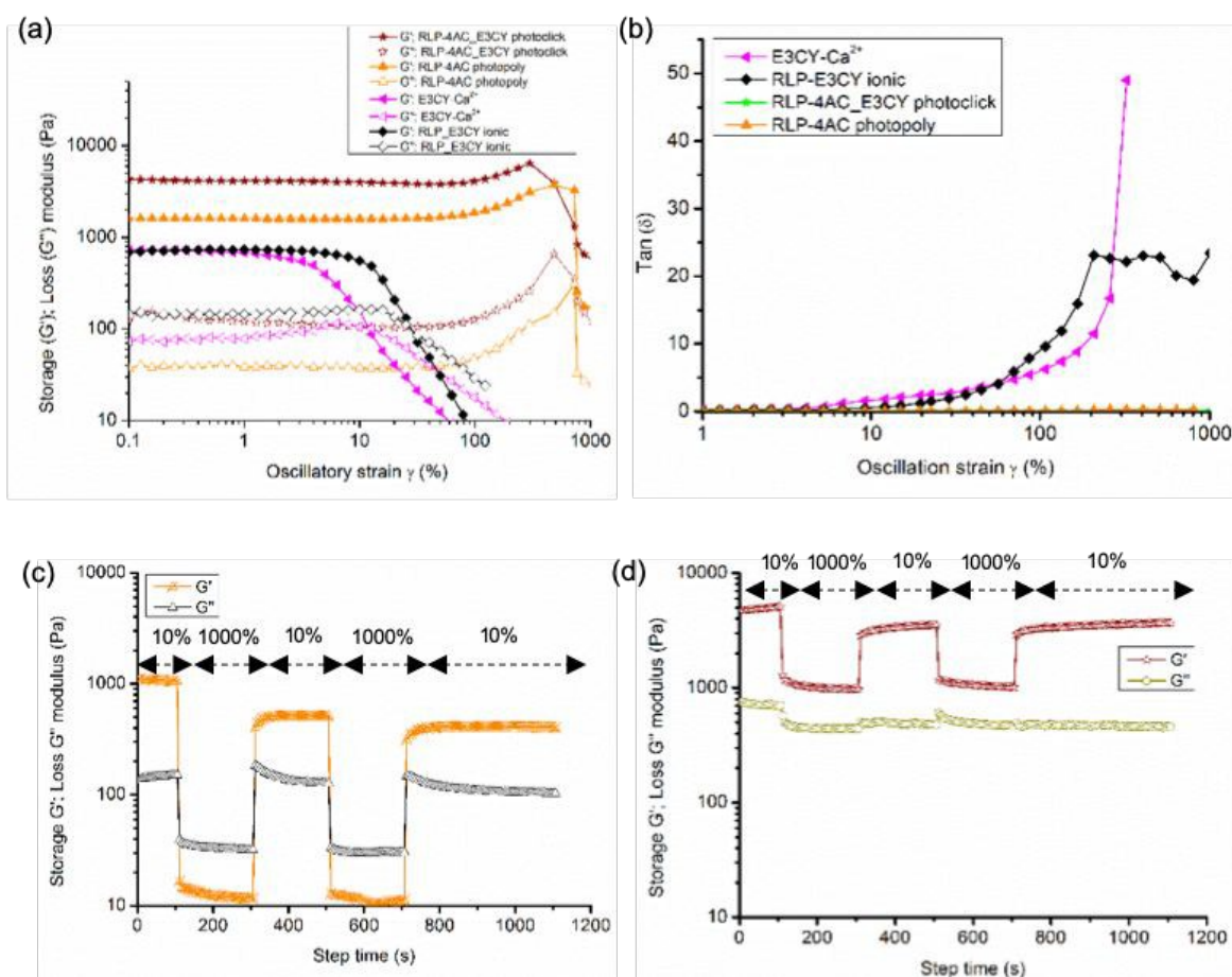
Figure 6. (a) Amplitude sweep rheographs for the photopolymerized RLP-4AC (10 wt %), E3CY- Ca 2+ (1 wt %), thiol-ene photoclicked RLP-4AC (20 wt %)_ E3CY (2 wt %), and RLP (20 wt %)_ E3CY (2 wt %). (b) \tan(\delta) versus strain rheographs for the photopolymerized RLP-4AC (10 wt %), E3CY-Ca 2+ (1 wt %) and thiol-ene photoclicked RLP-4AC (20 wt %)_ E3CY (2 wt %), and RLP (20 wt %)_ E3CY (2 wt %). Step-strain measurements with applied oscillatory strain alternated between 10 and 1000% for 100, 200, 200, 200 and 400 s ( f = 1 Hz, 20 °C) on (c) photopolymerized RLP-4AC and (d) photoclicked RLP-4AC_E3CY hydrogels.
