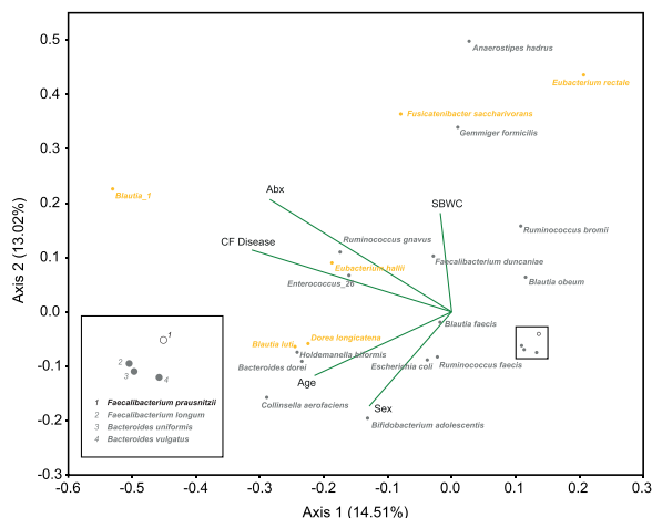
Fig. 3. Redundancy analysis species biplots for the whole microbiota. The 24 taxa contributing most to the dissimilarity (cumulatively > 50 %) between healthy control and pwCF samples following extended ETI therapy from the SIMPER analysis (Table 2) are shown independently of the total number of ASVs identified (531). Orange points represent taxa that were identified as core for the pwCF group following extended ETI therapy, grey points are satellite, and the white (black stroke) points represent taxa that were absent. Biplot lines depict clinical variables that significantly account for total variation in taxa relative abundance within whole microbiota analysis at the p \leq 0.05 level (Table 3). Species plots depict the strength of explanation provided by the given clinical variables, with taxa shown in the same direction of a particular clinical variable considered to have a higher value than those that are not. 'Abx' – Antibiotics during sampling period, 'SBWC' – Small bowel water content corrected for body surface area. The percentage of microbiota variation explained by each axis is given in parentheses.
