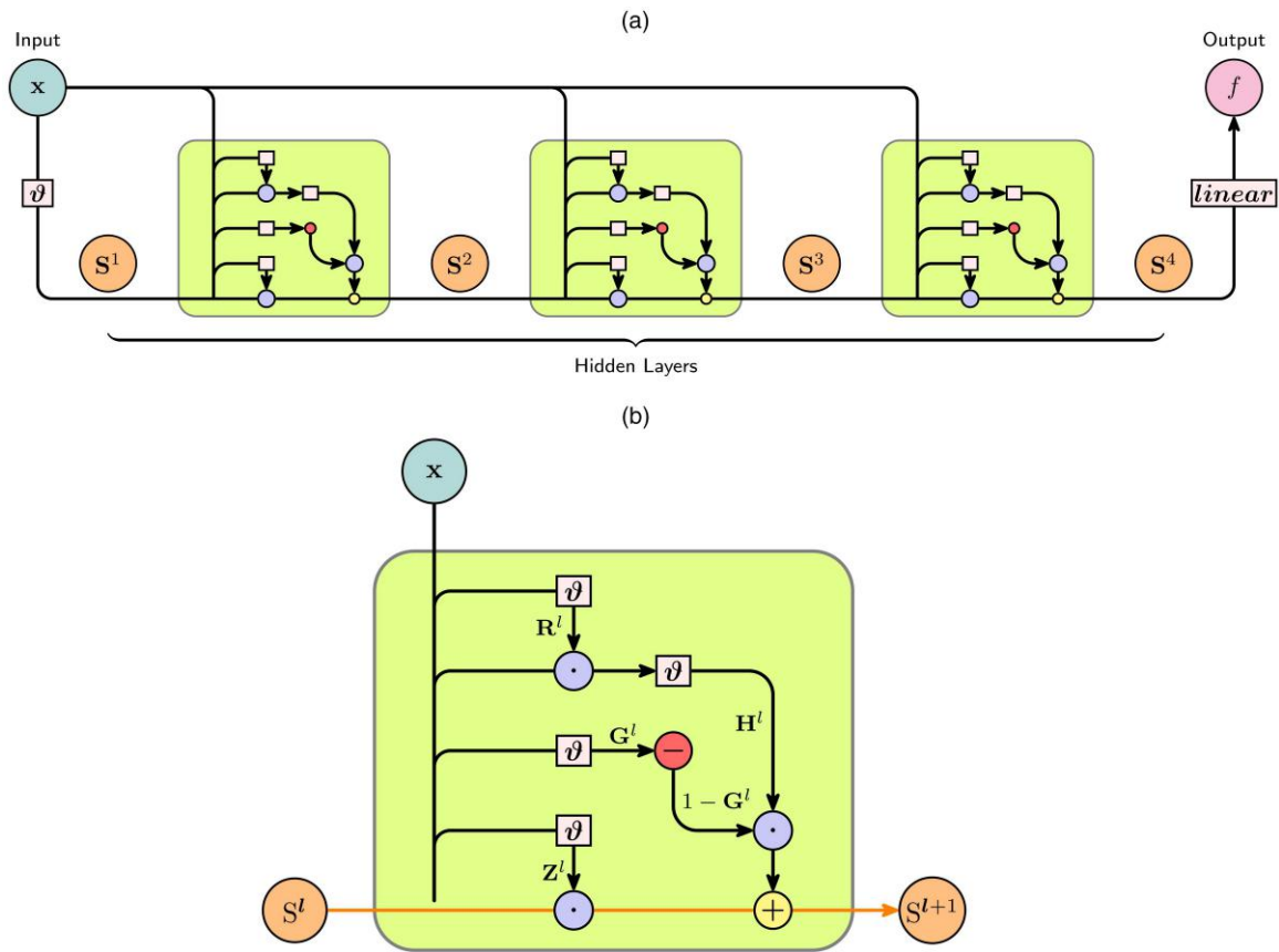
Figure 1. (Color online) Deep Galerkin Method NN Architecture Used in This Paper
