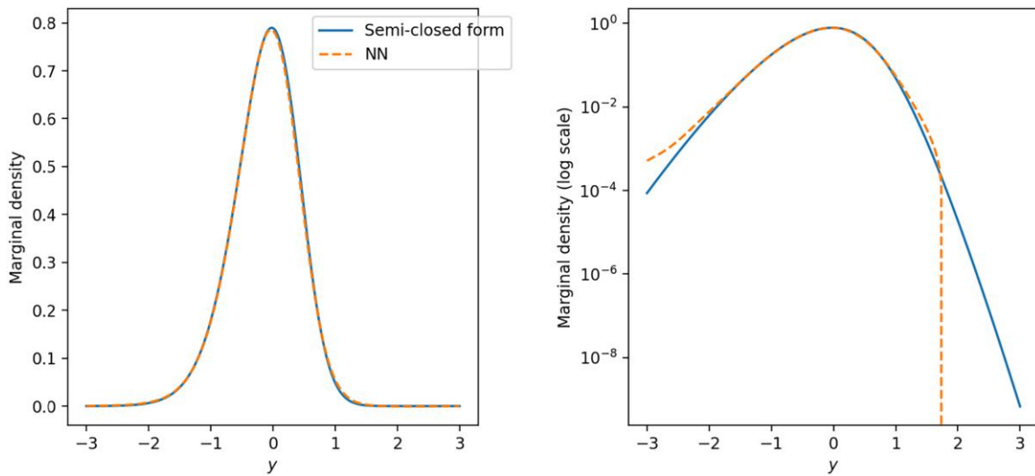
Figure 13. (Color online) SVJ Model Marginal Density Comparison: Semiclosed Form vs. NN
