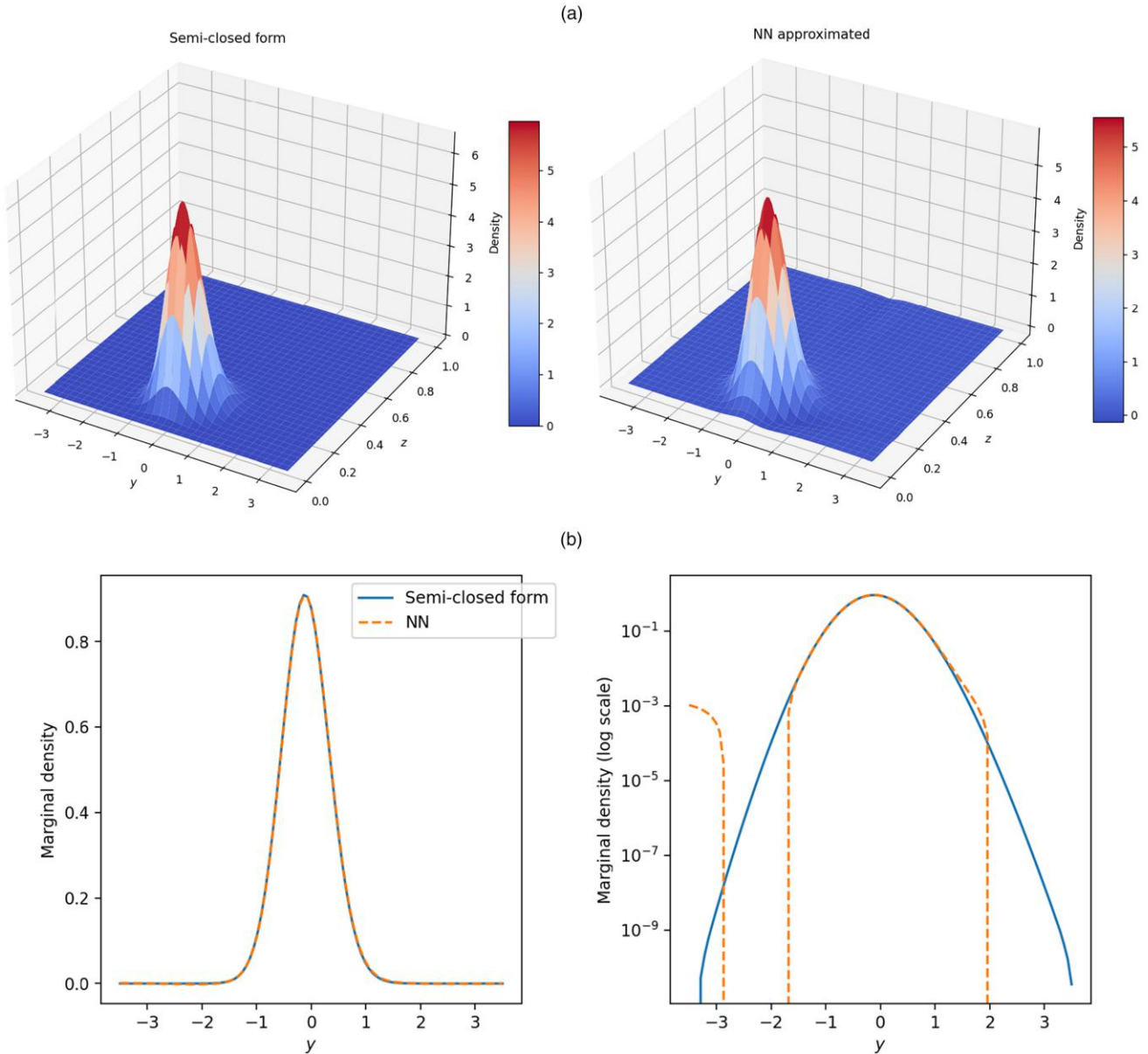
Figure 6. (Color online) Joint TPDF Graphs According to the Semiclosed Form and to the NN Approximation and Corresponding Marginal Densities
