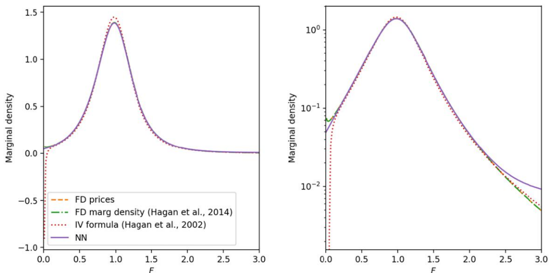
Figure 9. (Color online) Comparison of Marginal Densities for the SABR Model Calculated by Different Methods
