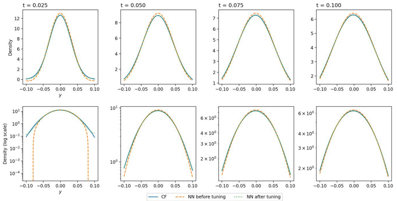
Figure 5. (Color online) The Exact Gaussian TPDF and the Neural TPDF Before and After Tuning for Small Time to Maturity
