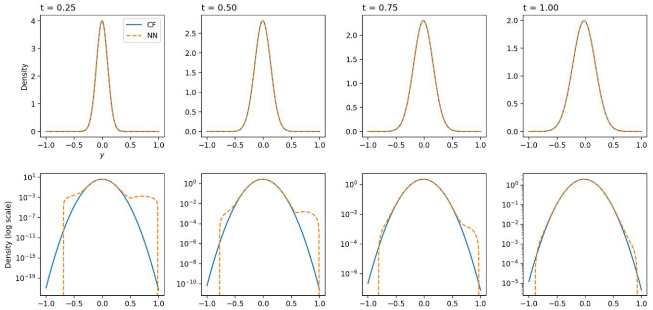
Figure 3. (Color online) Gaussian TPDF: Closed Form vs. NN Approximation
