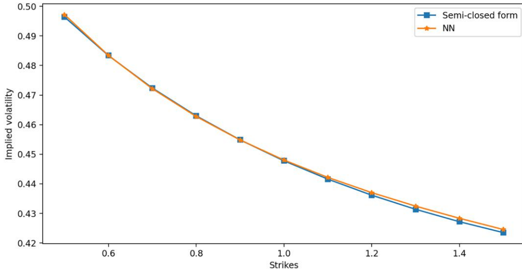
Figure 8. (Color online) Heston’s Volatility Smile Obtained Through Put Prices Under the Semiclosed Form TPDF and Neural TPDF
