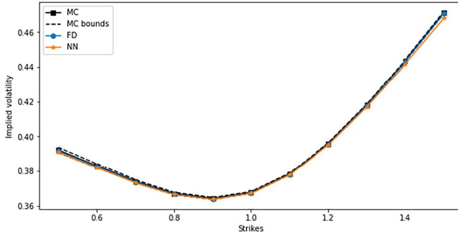
Figure 10. (Color online) SABR Volatility Smile Obtained Through Call Prices Using the QUAD Method with TPDF Computed Using Finite Difference Methods and with the Neural TPDF, Monte Carlo Simulations, and Approximate Implied Volatility Formula
