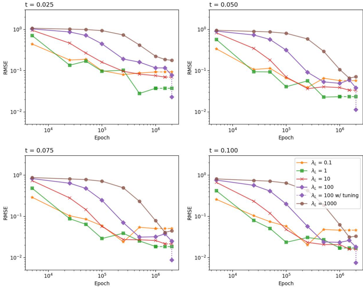
Figure 4. (Color online) RMSE Against Epoch for Different \lambda_L Across Various Small Times t Under the Black-Scholes-Merton Model
