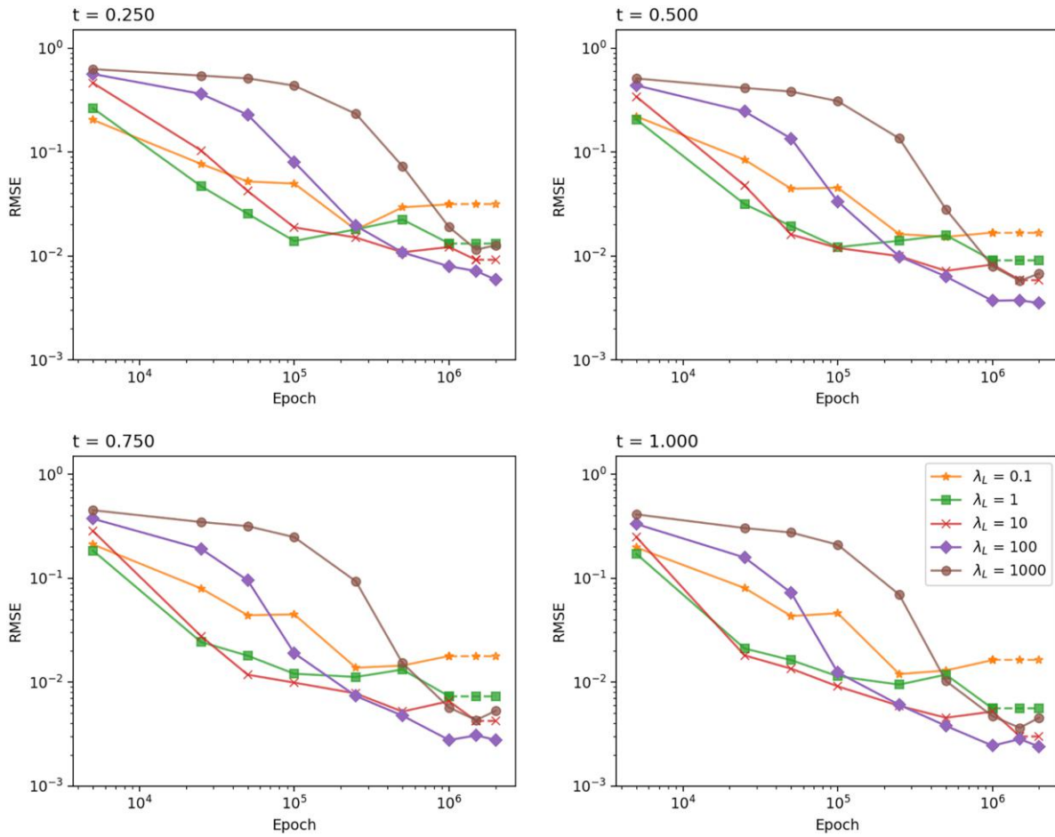
Figure 2. (Color online) RMSE Against Epoch for Different \lambda_L Across Various Times t Under the Black-Scholes-Merton Model
