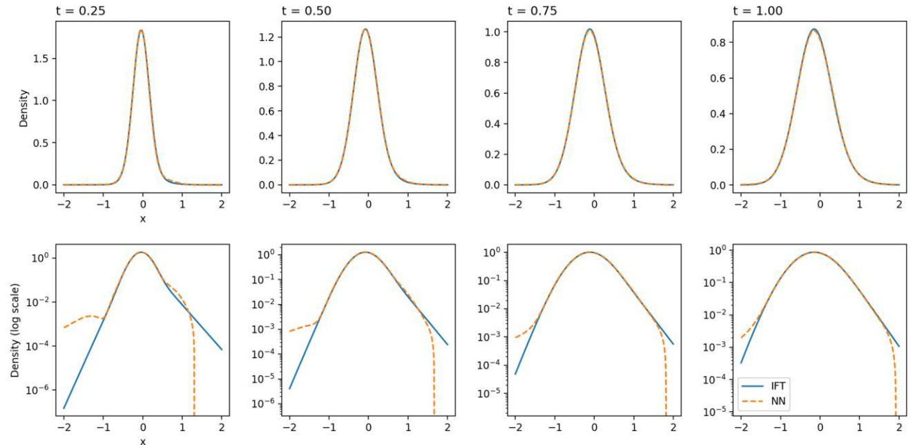
Figure 11. (Color online) True TPDF vs. Neural TPDF for Kou’s Double Jump Exponential Model
