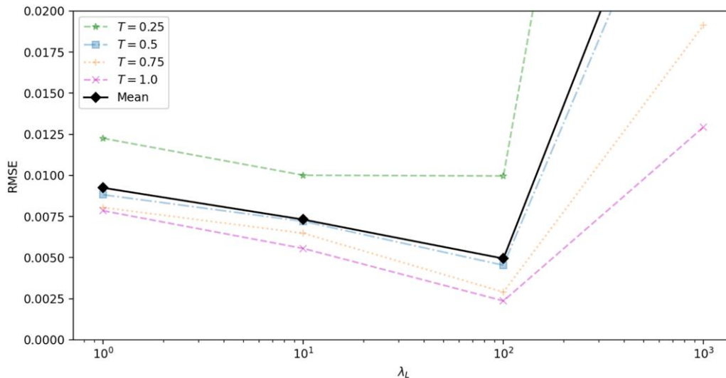
Figure 7. (Color online) RMSE Plot Against \lambda_L for the Heston Model with \lambda_L = 1, 10, 100, 1,000
