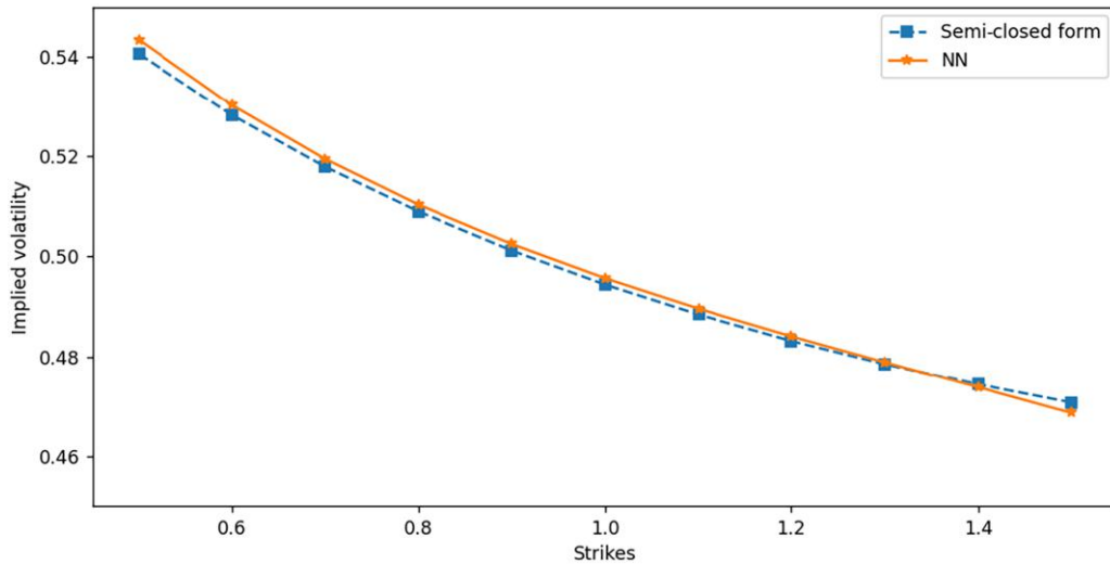
Figure 14. (Color online) SVJ Model Implied Volatility Smile Comparison: Semiclosed Form vs. NN
