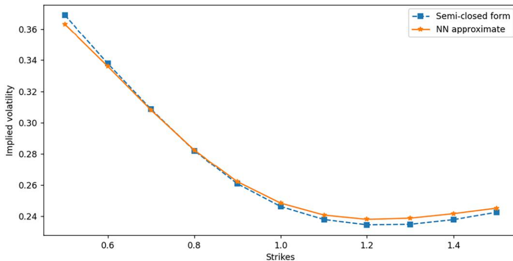
Figure 12. (Color online) Kou’s Double Exponential Jump Diffusion Volatility Smile Obtained Through Put Prices Using the Semiclosed Form European Option Pricing Formula (Kou 2002) and the QUAD Method with Neural TPDF
