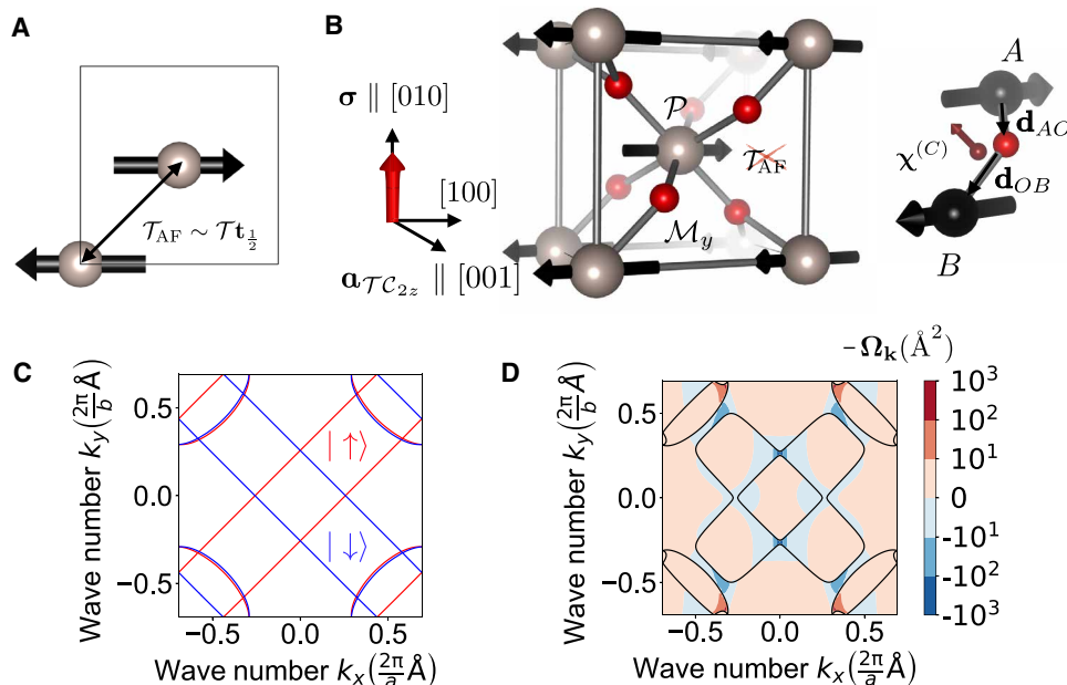
Fig. 2. Crystal symmetry breaking, large spin-split Fermi surface, and Berry curvature in collinear antiferromagnet \text{RuO}_2 . (A) Collinear antiferromagnet with effective time-reversal symmetry \mathcal{T}_{AF} . (B) Left: The unit cell of antiferromagnetic \text{RuO}_2 with the Néel vector along the [100] axis and marked crystal symmetries. Right: Detail of the generation of the local crystal chirality by noncentrosymmetric oxygen atoms \chi_{AB}^C \sim \mathbf{d}_{AO} \times \mathbf{d}_{OB} . (C) Antiferromagnetic Fermi surface cut at wave vector k_z = 0 calculated without spin-orbit coupling. The spin up and down projections are colored in red and blue. (D) Calculations with spin-orbit coupling of crystal momentum resolved Berry curvature \Omega_y(k_x, k_y, 0) in atomic units.
