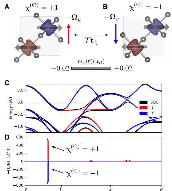
Fig. 3. Crystal chirality control of Hall conductivity sign. (A and B) View along the tetragonal crystal axis on the \text{RuO}_2 crystal with two possible configurations of nonmagnetic oxygen atoms. Redistribution of the oxygen atoms does not change the magnetic symmetry of the crystal; however, it changes the local crystal chirality orientation \chi^{(C)} and rotates, by 90^\circ , the shape of the magnetization density isosurfaces. (C) Calculated energy bands in the \text{RuO}_2 antiferromagnet without spin-orbit coupling (red and blue bands correspond to the opposite spin projections) and with spin-orbit coupling (black bands). (D) The largest contribution to the Berry curvature \Omega originates from the spin-split bands by the spin-orbit coupling. The red and blue color corresponds to the two opposite crystal chiralities \chi^{(C)} and demonstrates the expected Berry curvature sign change [compare to (A) and (B)].
