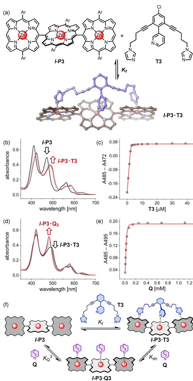
Figure 3. (a) Chelation of T3 to I-P3 ; optimized geometry of I-P3-T3 calculated by DFT (PBE0-D3(BJ)/Def2SVP); the Cl and aryl groups were replaced with hydrogen to simplify the calculation. Ar is 3,5-bis-(octyloxy)phenyl. (b) UV/Vis titration of I-P3 with T3 ( [\text{I-P3}]_0 = 3.0\text{ }\mu\text{M} , in \text{CDCl}_3 at 298 K). (c) Binding isotherm for formation of I-P3-T3 . (d) UV/Vis titration of I-P3-T3 with quinuclidine ( Q ). (e) Denaturation binding isotherm ( [\text{I-P3-T3}]_0 = 3.0\text{ }\mu\text{M} , in \text{CDCl}_3 at 298 K). In (b) and (d), the initial spectra are black and the final spectra are red. In (c) and (e), experimental points (black circles) and calculated binding isotherms (red line). (f) Thermodynamic cycle showing the formation and denaturation of I-P3-T3 . K_Q is the binding constant for porphyrin monomer and quinuclidine ( \log_{10} K_Q = 5.59 \pm 0.03 in \text{CDCl}_3 at 298 K).
