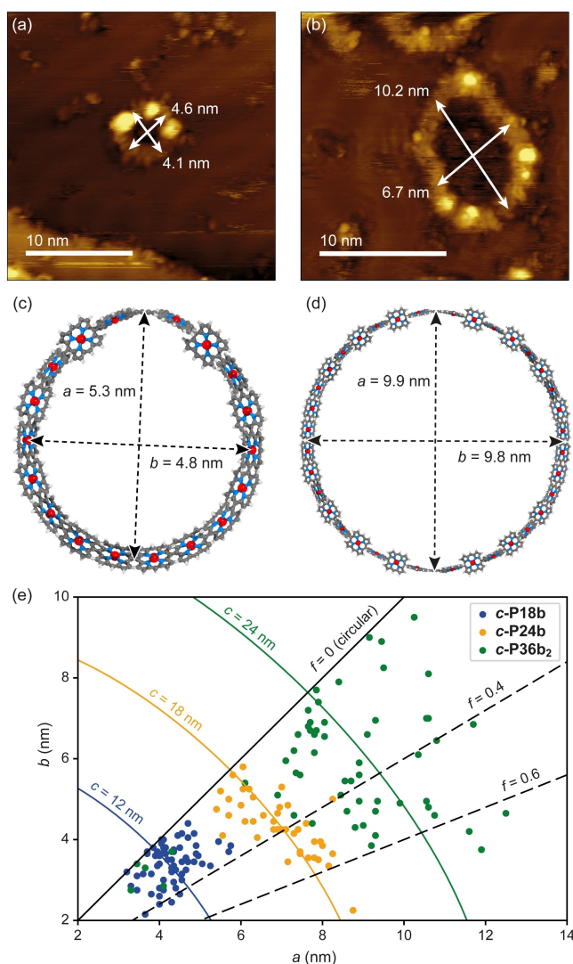
Figure 4. STM images of porphyrin nanorings c-P18b (a) and c-P36b 2 (b), deposited onto Au(111) via electro spray deposition. Imaging parameters: sample bias = -1.8 V, set-point current = 15 pA. Optimized geometry of c-P18b (c; PBE0-D3(BJ)/Def2SVP) and c-P36b 2 (d; PM7). Aryl and octyl groups were replaced by hydrogen to simplify the calculation. (e) Plots of experimentally measured long ( a ) versus short ( b ) axes of c-P18b (blue dots, 41 molecules), c-P24b (orange dots, 38 molecules), and c-P36b 2 (green dots, 59 molecules). f = 1 - b/a indicates the ellipticity or flattening factor of the nanorings. The blue, orange, and green arcs correspond to ellipses of fixed circumference calculated using the Ramanujan's approximations – the values are equivalent to the average circumference obtained for each nanorings. The solid black line indicates circular geometries ( a = b, f = 0 ). The dotted lines represent f = 0.4 and 0.6 , the shape becoming more elliptical with increasing f value.
