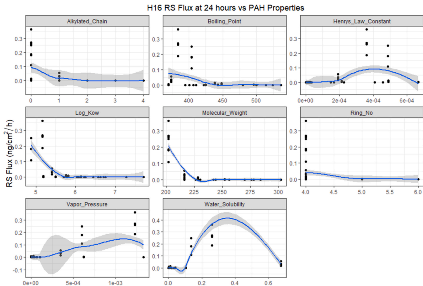
Fig. 7. Multiple plots of the sample H16 RS flux relationship with PAH physicochemical properties. The y-axis plots the H16 RS fluxes at 24-h for triplicate experiments and the x-axis plots the PAH physicochemical properties: alkylated chain length, boiling point ( ^{\circ}\text{C} ), Henry's Law Constant, Log Kow, Molecular weight (Da), number of rings in structure, vapour pressure (Pa) and water solubility (mg/L). Physicochemical property values taken from Achten and Andersson [2] whereby the mean physicochemical property values of individual alkyl-PAHs were used to represent the alkylated homologue series. Line of best fit calculated with locally estimated scatterplot smoothing (LOESS).
