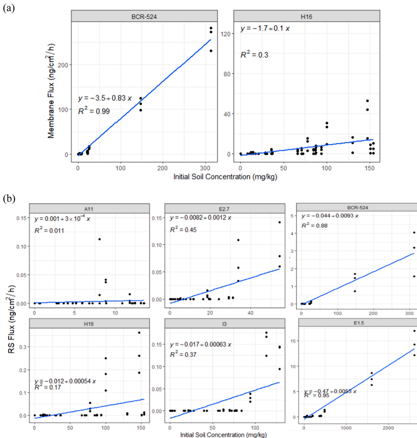
Fig. 8. The initial soil PAH concentration (mg/kg) of the 27 HMW PAHs plotted against (a) 24-h membrane fluxes for H16 and BCR-524 and (b) 24-h RS fluxes for all samples, line produced from linear regression.
