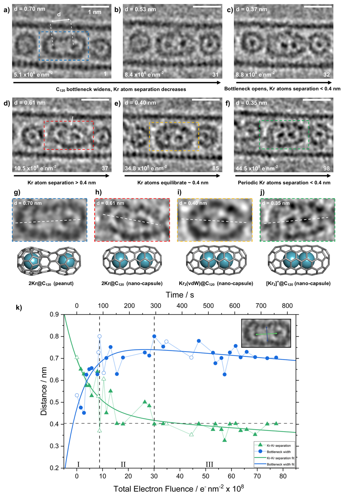
Figure 6. (a–f) Time-series AC-HRTEM images (80 kV; 1 \times 10^7 \text{ e}^- \text{ nm}^{-2} \text{ s}^{-1} ) illustrating the latter stages of coalescence of two Kr@C 60 molecules encapsulated within a SWCNT. Total electron fluence and frame number for each image is shown at the bottom of each panel, with Kr–Kr separations noted at the top left. (g–j) Enlarged views of (a), (d), (e), and (f), respectively, and accompanying structural models showing the relative position and bonding state of the Kr atoms. (k) Kr–Kr separation (green triangles) and C 120 bottleneck width (blue circles) for this time series, as a function of increasing time or electron fluence. Unfilled data points correspond to Figure 6a–f. Fitted curves for each data set are shown. The horizontal dashed line indicates the theoretical Kr–Kr van der Waals separation. Statistical data corresponding to dimerization event frequency is shown in Table S2.
