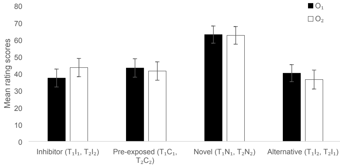
Figure 1. Mean rating scores (participants' expectancies) \pm SEM to the questions about O 1 and O 2 for the transfer cues in compound with the inhibitors (T 1 I 1 , T 2 I 2 ) the preexposed control cues (T 1 C 1 , T 2 C 2 ), the novel control cues (T 1 N 1 , T 2 N 2 ) and the alternative inhibitors (T 1 I 2 , T 2 I 1 ) in the summation test.
