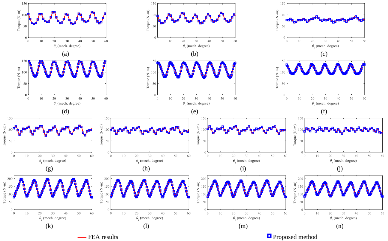
FIGURE 9. Comparison of the rated torque between FEA and the proposed method, considering (a), (b), (c) 4P1B machine (d), (e), (f) 6P1B machine; (g), (h), (i), (j) 4P2B machine, and (k), (l), (m), (n) 6P2B machine. Specifications of these scenarios can be found in Annex 1.
