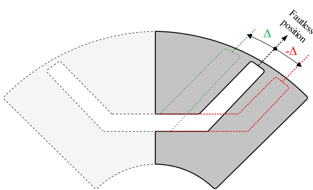
FIGURE 5. Schematics of possible failures with F = 2 on the right side of a barrier of a single pole.
