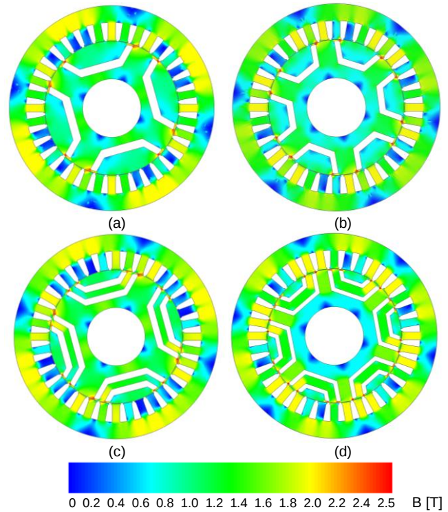
FIGURE 8. Flux density distribution of the selected machines without dimensional deviations: (a) four pole with one barrier; (b) six pole with one barrier; (c) four pole with two barrier; (d) six pole with two barrier.
