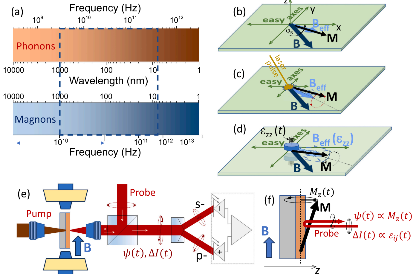
Fig. 1. Excitation and detection of coherent magnons and phonons in a metallic ferromagnet. (a) Frequencies and wavelengths of phonons and magnons in ferromagnetic metals. The dashed frame shows the typical range of frequencies and wavelengths excited by a femtosecond laser pulse in a ferromagnetic metal. (b)–(d) Used coordinate system and excitation of the magnetization precession: (b) equilibrium state with the magnetization, \mathbf{M} , along the effective field, \mathbf{B}_{\text{eff}} , defined by the balance of the external magnetic field, \mathbf{B} , and the anisotropy field, which defines the easy axes of magnetization; (c) ultrafast tilt of \mathbf{B}_{\text{eff}} due to the rapid decrease of the anisotropy field, induced by the femtosecond laser pulse, followed by precession of \mathbf{M} ; (d) phonon-induced precession by a quasi-harmonic modulation of \mathbf{B}_{\text{eff}} via dynamical strain. (e) Experimental scheme, in which a metallic ferromagnetic film is excited from the backside through the transparent substrate. The transient Kerr rotation and reflectivity signals, \psi(t) and \Delta I(t) , given by the z-projection of the precessing magnetization and the dynamical strain, respectively, as illustrated in (f). The signals are measured by a balanced photoreceiver as the difference [\psi(t)] and the sum [\Delta I(t)] of the intensities of the pulses of orthogonal polarizations, split from the linearly polarized probe pulse by a Wollaston prism.
