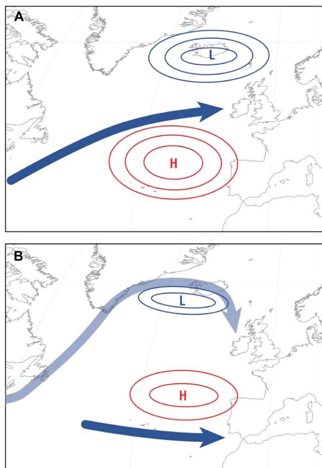
Figure 8. Cartoon representing possible atmospheric circulation during (A) the Early Holocene and (B) the Mid-Holocene to explain trends in carbonate oxygen isotope values in the lakes in this study and in northern Sweden (in Hammarlund et al., 2002). H and L = high and low surface pressure, respectively. Blue arrows mark the approximate position and strength (dark blue = stronger, light blue = weaker) of the jet stream in the upper atmosphere, and trajectory of storm tracks. [Color figure can be viewed at wileyonlinelibrary.com ]
