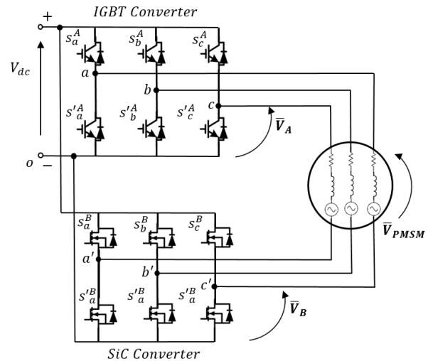
Fig. 1. Dual-Fed single dc-link OEW-PMSM with mixed technology VSCs.
