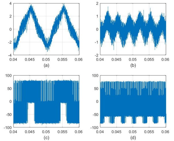
Fig. 11. Speed \omega_m of 2000 rpm. Standard PWM. (a) Phase current i_a . X-axis: 5ms/div; Y-axis: 2 A/div (b) ZSC i_0 . X-axis: 5ms/div; Y-axis: 1 A/div (c) Phase voltage V_{aa'} . X-axis: 5ms/div; Y-axis: 50 V/div (d) ZSV V_0^{PMSM} . X-axis: 5ms/div; Y-axis: 50 V/div
