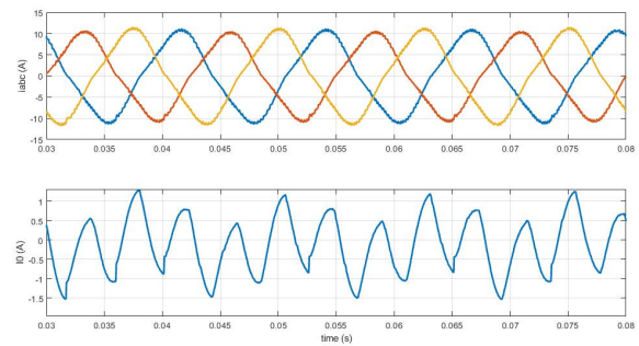
Fig. 14. Experimental results at \omega_m of 1600 rpm and increased load torque. Top: Phase current i_a, i_b, i_c (blue, red, and yellow respectively). Bottom: ZSC i_0 .
