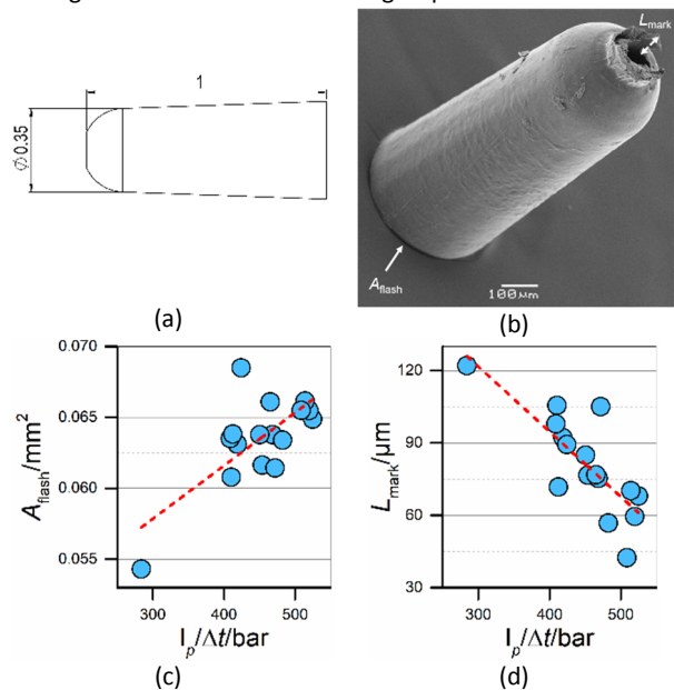
Figure 2. (a) Micro part main dimensions; (b) \mu\text{IM} part, gate mark and flash; (c) A_{\text{flash}} product vs process fingerprint; (d) L_{\text{mark}} product vs process fingerprint. The red dashed line represent the linear regression trend.
