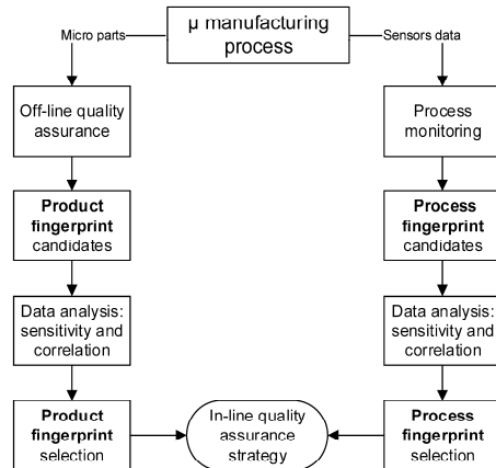
Figure 1. Flowchart representing the method to identify product and process fingerprints leading to the definition of an in-line quality assurance strategy.
