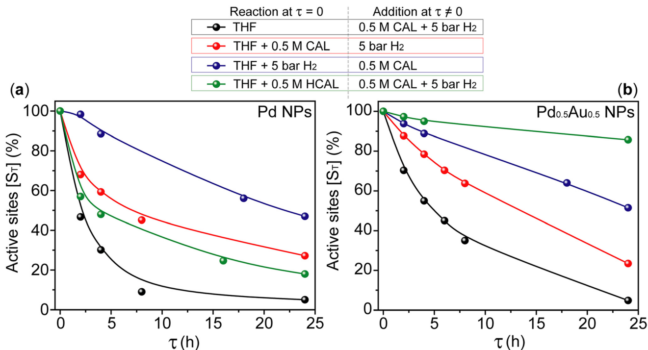
Fig. 4 Dependence of the relative concentration of total available sites [S T ] on the incubation time \tau for (a) Pd NPs and (b) Pd 0.5 Au 0.5 NPs in the presence of only THF (black), in the presence of 0.5 M HCAL (green), in the presence of 0.5 M CAL (red), and under 5 bar H 2 (blue). In all experiments, it was assumed that the catalyst deactivation takes place only during the incubation period, thus the initial rates are not affected by further catalyst deactivation. The relative concentration of available sites was estimated using the fraction of the initial rate after the incubation period and the initial rate at \tau = 0 (see ESI† for further details).
