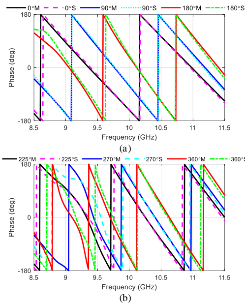
Fig. 10. The measured S_{21} of the proposed non-uniform LM phase shifter. (a) 0° to 180° and (b) 180° to 360°. [M: is for measurement results and S is for simulated results]
