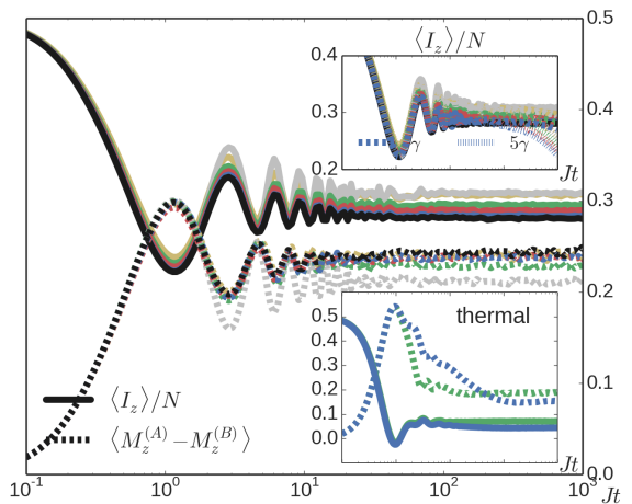
FIG. 8. Observable averages in MBL and thermal phases: imbalance (solid lines) and average half-chain magnetizations difference (dashed lines) for the XXZ chain of Sec. V. They both show a quick approach to stationarity for, in contrast to the behavior of quantum correlations (cf. Fig. 5). In particular, there is no appreciable difference in timescales between the interacting and noninteracting cases. The parameters of the dynamics [cf. Eqs. (54) and (58)] are N = 6, 8, 10, 12, 14 [yellow, green, red, blue, and black (grayscale: light gray to black), respectively; open case only up to N = 12 ], V/J = 2 and h/J = 5 ; gray (top solid and bottom dashed) curves are for V/J = 0 and N = 8 . The bottom inset shows that in the thermal phase ( V/J = 2 and h/J = 1 ) the asymptotic values decrease with the system size [green (gray) N = 8 and blue (darker gray) N = 12 ]. The top inset shows that the average imbalance in the presence of dephasing \gamma/J = 2 \times 10^{-4} (dashed curves) and 10^{-3} (dotted curves) decays to zero.
