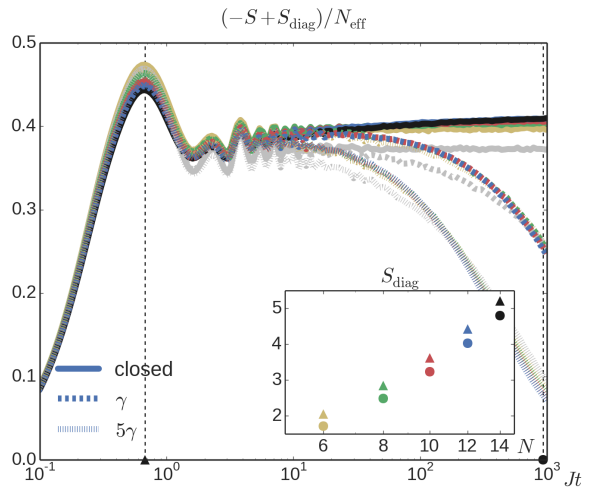
FIG. 4. Coherence as an upper bound on the MPE in an MBL system. We show coherence (10), which is a faithful upper bound on MPE, cf. Eq. (38), for the XXZ chain of Sec. V. The curves are rescaled by the effective system size N_{\text{eff}} = \log_2 \binom{N}{N/2} of the zero z magnetization subspace. In the presence of dephasing, coherence decays at a rate proportional to the dephasing strength \gamma and is weakly dependent on the interaction strength, but not on the system size. The inset shows that the coherence in the closed dynamics ( \gamma = 0 ) at t = 1/J (triangles) and t = 10^3/J (circles) follows the same scaling with system size. The parameters of the dynamics [cf. Eqs. (54) and (58)] are N = 6, 8, 10, 12, 14 spins [yellow, green, blue, red, black (grayscale: light gray to black), respectively], V/J = 2 , h/J = 5 , and \gamma/J = 2 \times 10^{-4} ; gray (bottom) curves are the noninteracting case V/J = 0 with N = 8 (here results are independent of system size as entanglement obeys the area law).
