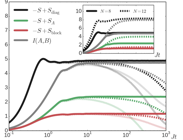
FIG. 12. Correlations in the thermal phase of an MBL system: relative entropy coherence (10) [black (top) curve], a lower bound on the relative entropy of entanglement [113] -S(\rho) + S(\rho_A) [green (lower middle) curve], half-chain magnetization asymmetry (15) [red (bottom) curve], and mutual information (total classical and quantum correlations) I = (A, B) \equiv S(\rho_A) + S(\rho_B) - S(\rho) [gray (upper middle) curve] in thermal phase of MBL system ( V/J = 2 , h/J = 1 , and N = 8 ). Solid lines corresponds to the closed case, while the open case with dephasing is illustrated by dashed ( \gamma/J = 2 \times 10^{-4} ) and dotted ( \gamma/J = 10^{-3} ) lines. The inset shows the closed case for N = 8 (solid lines) and N = 12 (dashed lines) spins.
