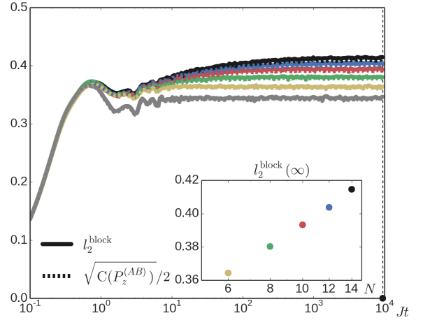
FIG. 11. Experimentally accessible lower bounds on BPE in an MBL system. We show the dynamics of l_2^{\text{block}}(\rho) (solid lines) and C(P_z^{(AB)}, \rho) , where the parity P_z^{(AB)} \equiv (-1)^{\delta M/2} for the XXZ disordered chain of N = 6, 8, 10, 12, 14 spins [yellow, green, red, blue, and black (grayscale: light gray to black), respectively]. The inset shows asymptotic values of l_2^{\text{block}}(\rho) at Jt = 10^4 . Parameters of the dynamics (54) and (58) are V/J = 2 , h/J = 5 and \gamma/J = 0 , while the gray (bottom) curves corresponds to the noninteracting case V/J = 0 and N = 12 .
