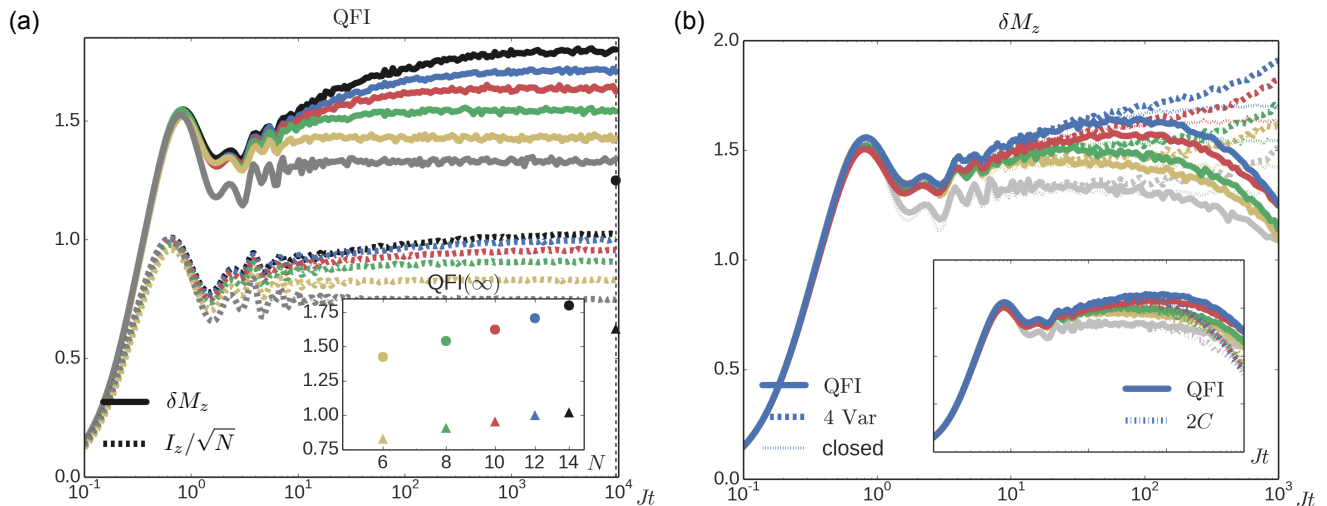
FIG. 3. Witnessing bipartite entanglement in an MBL system with conserved charge. We show for the XXZ chain of Sec. V that not only MPE can be witnessed, but also BPE, provided that the phase encoding observable commutes with subsystem charges Q^{(A)} and Q^{(B)} in the bipartition. (a) For closed dynamics ( \gamma/J = 0 ) the QFI of the z -magnetization difference between two halves of the chain (solid lines) witnesses BPE at all times t > 0 . Similarly, the QFI of the z imbalance (dashed lines) witnesses BPE in the staggered partition ( ABAB \dots AB instead of AA \dots AB \dots BB ) at all times t . The inset shows that asymptotic values (taken from Jt = 10^4 ) of the QFI for the z -magnetization difference (circles) and the z imbalance (triangles), as a function of size N , grow with system size (cf. Ref. [43]). For the z imbalance the asymptotic value grows with N even after rescaling by the system size. (b) In the presence of local dephasing ( \gamma/J = 2 \times 10^{-4} ) the QFI of the magnetization difference (solid lines) decays in comparison with the closed case (dotted lines), while the variance (dashed line) increases, thus overestimating the QFI [cf. Eq. (A7)]. The inset shows that both the QFI (solid lines) and its lower bound in terms of the curvature (dotted lines) (defined in Appendix A) witness BPE for the observable chosen as the magnetization difference, although the curvature decays at faster rate dependent on the system size [40, 64]. The parameters of the dynamics [cf. Eqs. (54) and (58)] are N = 6, 8, 10, 12, 14 [yellow, green, red, blue, and black (grayscale: light gray to black), respectively, open case only up to N = 12 ], V/J = 2 , h/J = 5 , and \gamma/J = 2 \times 10^{-4} ; gray (bottom) curves correspond to the noninteracting case V/J = 0 with N = 12 (closed dynamics) and N = 8 (open dynamics). Here the QFI is independent of system size as entanglement obeys the area law.
