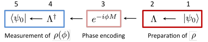
FIG. 10. Protocol for the curvature and the MQC spectrum. For a system state \rho being a result of dynamics from |\psi_0\rangle (steps 1 and 2), its coherence with respect to the eigenbasis of an observable M can be accessed by unitary perturbation encoding a phase \phi (step 3), followed by a measurement (step 4 and 5) of the overlap between \rho(\phi) and the unperturbed state \rho . This measurement scheme can also be used to estimate the encoded phase value \phi , and in the case of (noninteracting) closed dynamics it corresponds to Ramsey spectroscopy [142].
