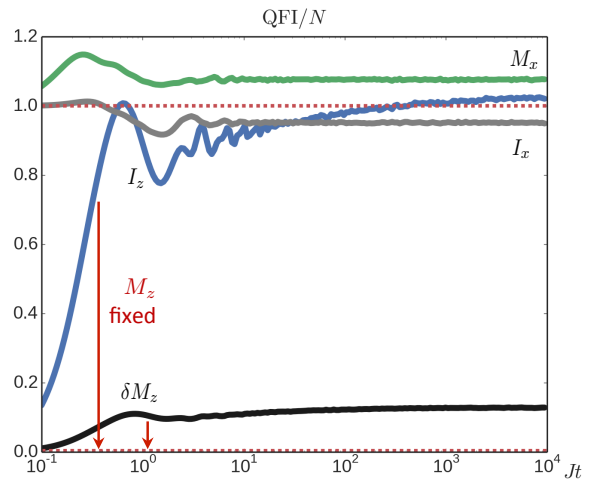
FIG. 2. QFI in an MBL system. Throughout the paper we illustrate our results with the example of a many-body localized system, an XXZ chain with strong disordered longitudinal field (see details in Sec. V). The figure shows the evolution of the QFI per number of subsystems N . We consider four different phase encodings: x magnetization M_x \equiv \sum_{k=1}^N S_k^x [green (top) line], the difference of z magnetization between two halves of the chain, \delta M_z \equiv \sum_{k=1}^{N/2} S_k^z - \sum_{k=N/2+1}^N S_k^z [black (bottom) line], and x and z imbalance I_{x,z} \equiv \sum_{k=1}^N (-1)^k S_k^{x,z} [blue and gray (at Jt = 10^{-1} lower and upper middle) lines, respectively]. The QFI witnesses entanglement only if the corresponding separability threshold \text{QFI}_{\text{sep}}/N = 1 [red dashed (horizontal) line] is crossed, cf. Eq. (9). Due to the conservation of M_z by the dynamics, for an initial state with a fixed M_z , the spin axes x and y are equivalent (and the QFI for M_y and I_y is equal to that the QFI for M_x and I_x , respectively). For observables commuting with M_z (here \delta M_z and I_z ) the separability threshold is reduced to zero, see Sec. III. The parameters of the dynamics [cf. Eqs. (54) and (58)] are N = 14 spins, V/J = 2 , h/J = 5 , and \gamma/J = 0 .
