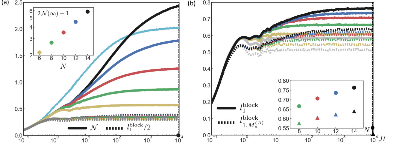
FIG. 6. Negativity and experimentally accessible lower bound in a closed MBL system. (a) We show the negativity of entanglement (Eq. (52)) for the XXZ chain of Sec. V. The negativity (solid lines) initially follows an area law for times Jt < 2 (with coefficient dependent on the interaction strength for Jt > 1 ), but at later times becomes dependent on the system size. The lower bound by l_1^{\text{block}} (Eq. (53)) is also shown (dashed lines) (cf. Fig. 7). The inset shows that the asymptotic values of \mathcal{N} in the closed dynamics (at Jt = 10^4 ) scales exponentially with the system size N (note the logarithmic scale of the vertical axis). (b) We show the lower bounds l_1^{\text{block}} \geq l_{1, M_z^{(A)}}^{\text{block}} on the convex roof of the negativity of entanglement (cf. Eq. (53)). Both l_1^{\text{block}} (solid lines) and the experimentally accessible l_{1, M_z^{(A)}}^{\text{block}} (dashed lines) initially follow the area law for times Jt < 2 , and at later times become dependent on the system size. In particular, the asymptotic value of l_1^{\text{block}} for the noninteracting system (gray) is crossed by l_{1, M_z^{(A)}}^{\text{block}} for sizes above N = 8 . The inset shows that the asymptotic values of l_1^{\text{block}} (circles) and l_{1, M_z^{(A)}}^{\text{block}} (triangles) in the closed dynamics (at Jt = 10^4 ) increases with the system size. The parameters of the dynamics [cf. Eqs. (54) and (58)] are N = 6, 8, 10, 12, 14 spins [yellow, green, red, blue, and black (grayscale: light gray to black), respectively], V/J = 2 and h/J = 5 ; gray (bottom) curves correspond to the noninteracting case V/J = 0 with (a) N = 12 and (b) N = 8 . Light-blue stars in (a) correspond to a more strongly interacting system with V/J = 5 and N = 12 .
