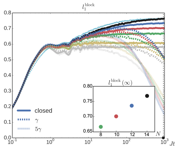
FIG. 7. Lower bound on BPE in an open MBL system. We show the lower bound on the convex roof on the negativity of entanglement by l_1^{\text{block}} [cf. Eq. (53)] for the XXZ chain of Sec. V. The solid curve is for the closed case and the dashed curves for the dissipative case. Decay in the presence of dephasing depends on both the system size and interaction strength. The inset shows that the asymptotic value of l_1^{\text{block}}(\rho) in the closed dynamics at t = 10^3/J (circles) grows approximately linearly with N (for N = 8, 10, 12, 14 ). The parameters of the dynamics [cf. Eqs. (54) and (58)] are N = 6, 8, 10, 12, 14 spins [yellow, green, red, blue, and black (grayscale: light gray to black), respectively, open case only up to N = 12 ], V/J = 2 , h/J = 5 , and \gamma/J = 2 \times 10^{-4} ; gray curves correspond to the noninteracting case V/J = 0 with N = 12 (closed dynamics) and with N = 8 (open dynamics) (here results are independent of system size as the system follows an area law). Light-blue stars in (a) correspond to a more strongly interacting system with V/J = 5 and N = 12 .
