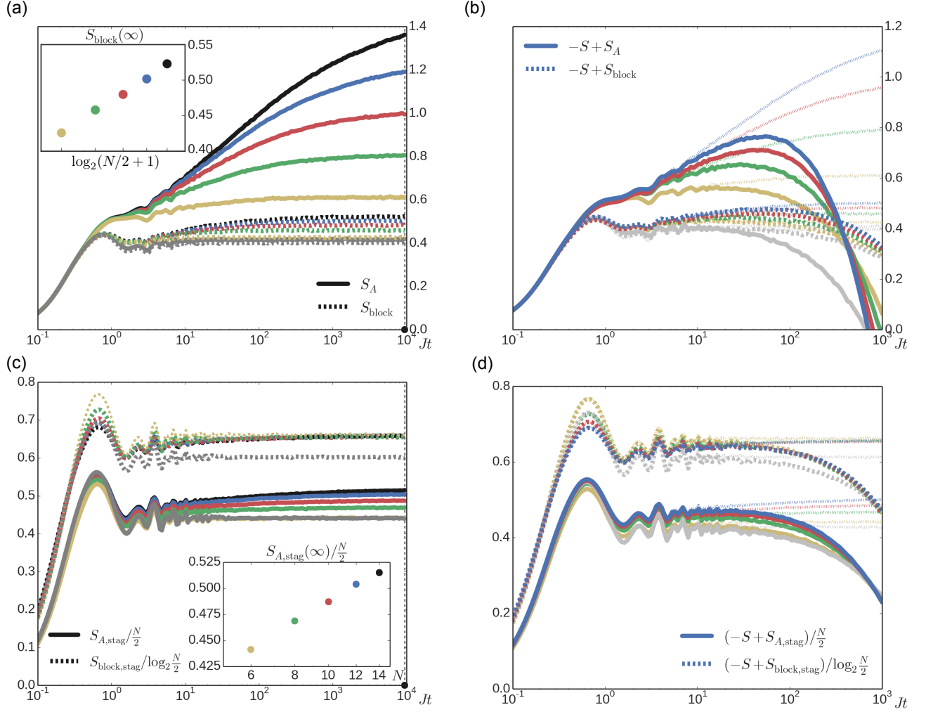
FIG. 5. Bipartite entanglement and asymmetry in an MBL system. (a) Entanglement entropy S(\rho_A) (solid lines) and asymmetry S_{\text{block}} of half-chain magnetization (dashed lines), [cf. (46)] for the XXZ chain of Sec. V, with closed dynamics. The asymmetry initially follows the area law ( Jt < 1 ), which is broken at later times, in analogy with the entanglement entropy. The inset shows the asymptotic value of the asymmetry (taken from Jt = 10^4 ) scales as \log_2(N/2 + 1) with system size (cf. Fig. 9). (That of the entanglement entropy, not shown, scales as N , as expected.) (b) Similar, but with dephasing, so for -S(\rho) + S_{\text{block}} (solid lines) and -S(\rho) + S(\rho_A) (dashed lines). Here the decay rate of the asymmetry is independent of the system size, but depends on the interaction strength (cf. Fig. 9). (c) Entanglement entropy (solid lines) for the staggered bipartition ( ABAB \cdots AB instead of AA \cdots AB \cdots BB ) and corresponding asymmetry of the staggered magnetization. The curves are scaled by N/2 and \log_2(N/2) , respectively. The inset shows that the asymptotic value of the entanglement entropy per site (taken from Jt = 10^4 ) displays an additional weak dependence on N . (d) Same as (c) but for the dissipative case (subtracting the von Neumann entropy S ). In the presence of dephasing, the decay of both sets of curves is independent of the system size, but depends on the interaction strength. The parameters of the dynamics [cf. Eqs. (54) and (58)] are N = 6, 8, 10, 12, 14 [yellow, green, red, blue, and black (grayscale: light gray to black), respectively, open case only up to N = 12 ], V/J = 2 , h/J = 5 , and with \gamma/J = 2 \times 10^{-4} for the dissipative case [(b) and (d)]; gray (bottom) curves correspond to the noninteracting case V/J = 0 and N = 12 (closed dynamics) and N = 8 (open dynamics), but in both cases the results follow area laws.
