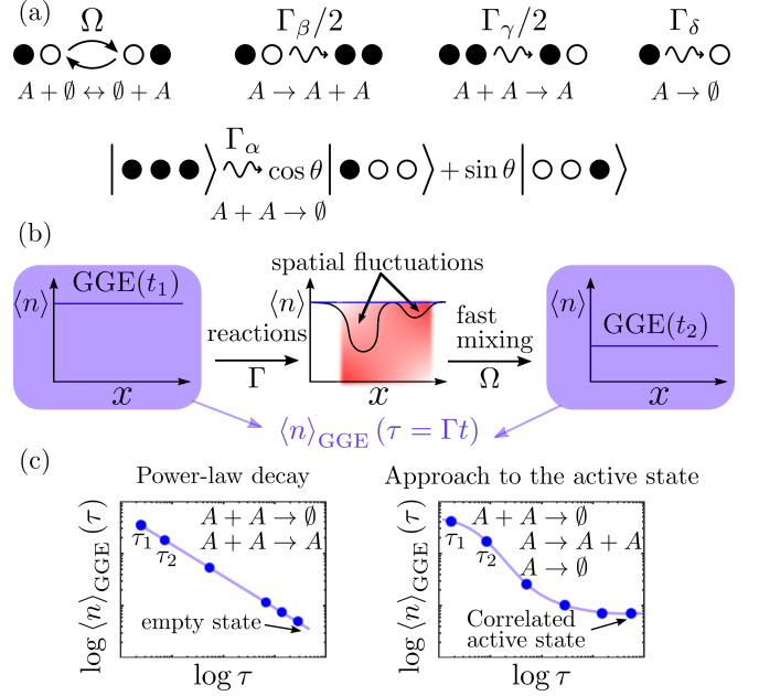
Figure 1. Quantum RD dynamics in the reaction-limited regime. (a) Quantum chain with sites that can either be occupied by a fermion, |\dots \bullet_j \dots\rangle , or empty |\dots \circ_j \dots\rangle . Particles can hop between nearest-neighboring sites with hopping rate \Omega , Eq. (2). Dissipation consists of irreversible reactions at rate \Gamma_\nu , Eqs. (4)-(6). The parameter \theta controls coherent superposition from pair annihilation events. (b) In the reaction-limited regime, \Gamma \ll \Omega , reaction dynamics is slow and takes place on the timescale \sim \Gamma^{-1} . Fast hopping rapidly smooths out spatial fluctuations (highlighted in red), due to local reactions, and the state of the systems is described by a homogeneous GGE( \tau ) (blue horizontal lines) at any rescaled time \tau = \Gamma t . (c) The total particle density \langle n \rangle_{\text{GGE}}(\tau) decays algebraically in rescaled time \tau (blue points) for annihilation or coagulation with exponent dependent on initial state coherence. When branching is included an absorbing-state phase transition to an active, finite density of particles, state can occur. The latter displays correlation when \theta \neq 0, \pi/2 .
