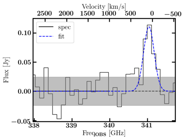
Figure 3. The same as in Fig. 2, but for the SHeFI-APEX2 spectrum targeting CO(6–5) transition.
