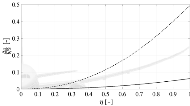
Figure 3. Trim state wing deformations for rigid (–) and flexible (– –) wing aircraft. The shape of Boeing 787 aircraft in trimmed flight (Dodt, 2011) is given for illustration purpose.
