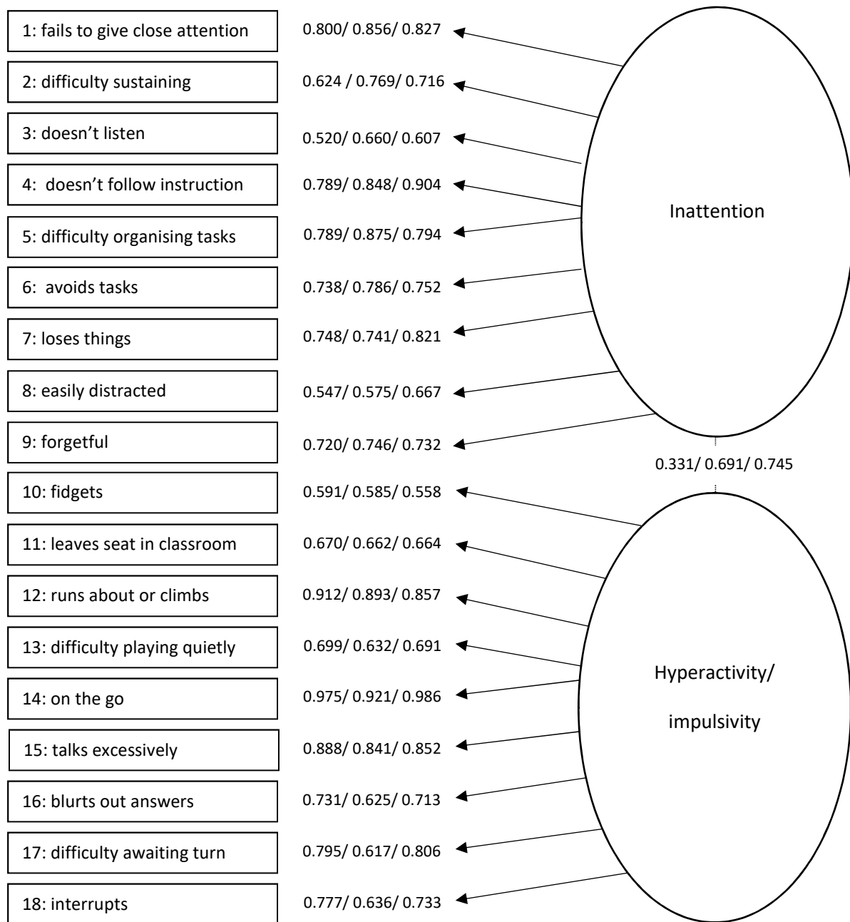
Figure 1: item factor loadings and correlations for baseline/follow-up parent
