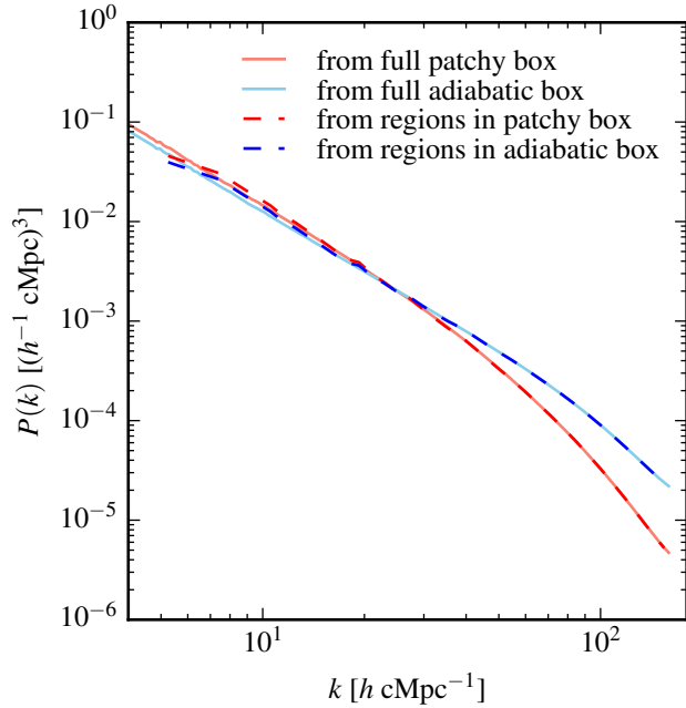
Figure B1. Gas density contrast power spectrum either calculated from a grid covering the full simulation box (solid lines) or by averaging the power spectra measured in all 32768 randomly placed regions (dashed lines). Results are shown for both the z_r = 5.3 patchy and the adiabatic simulation at z = 4.8 . The averages of the local power spectrum measurements are in excellent agreement with the corresponding globally computed power spectrum.
