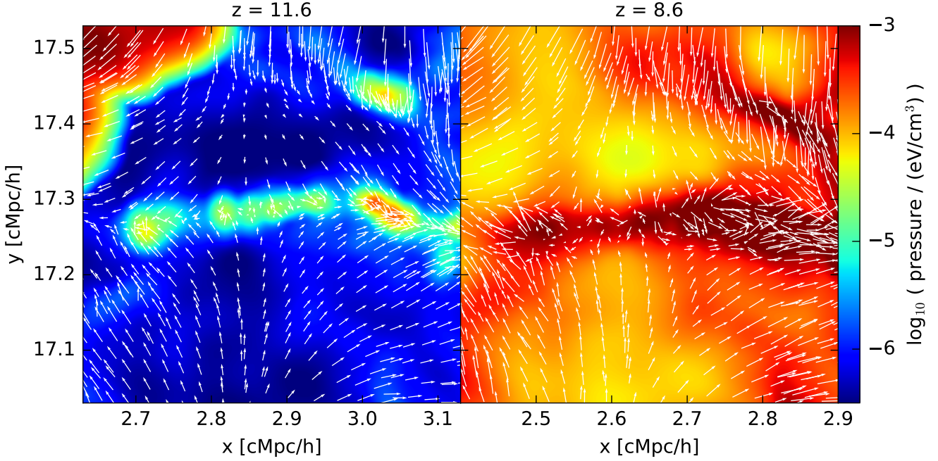
Figure 9. Gas pressure in thin slices through the z_r = 5.3 patchy simulation. Results are shown at z \approx 11.6 (left panel), when the region is still largely neutral (only the upper left corner has already been swept over by the approaching ionization front), and at z \approx 8.6 (right panel), after the region has been reionized. Both panels show the same structures, although note that different x -coordinate ranges have been used because the whole region is falling (almost exactly) towards the left. The arrows indicate the gas velocity in a reference frame in which the central filament is roughly at rest. The photoheating during reionization strongly boosts the gas pressure. This also increases the absolute difference in pressure between dense structures and voids. After reionization these structures are over-pressurized and start to expand, which is visible in the velocity fields. The gas velocities near the edge of the filament point inward before reionization, but outward after reionization. The arrows are scaled such that a velocity of 10 km/s corresponds to a length of 20 ckpc/h.
