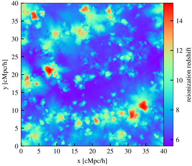
Figure 1. Map of the local reionization redshift in a thin slice produced by the radiative transfer calculation with the ATON code. This map corresponds to the z_r = 5.3 patchy simulation that is discussed later in the manuscript. For comparison, the large scale structures in the same slice are shown in Fig. 2.
