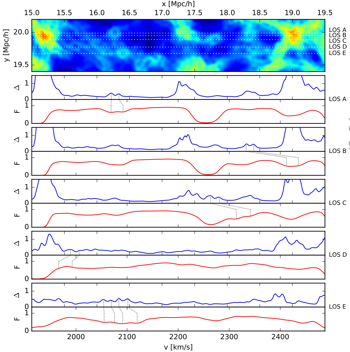
Figure 14. Expansion of gas overdensities due to the heating provided by reionization and their imprint on Lyman- \alpha forest absorption lines. The top panel displays the gas density in a thin slice in our z_r = 5.3 patchy simulation at z = 4.2 . Also indicated are five lines-of-sight (LOS A-E) for which we explore the Lyman- \alpha transmission. The five other sets of panels show the density (in units of the mean) and the normalized transmitted flux for these five lines-of-sight. In the top panel various “rings” are visible. These appear when the slice cuts through expanding spherical or cylindrical shells that are produced when overdensities are evaporated by the photoheating provided by reionization. In the density skewers, these “rings” are visible as pairs of density peaks. Some of them are marked by gray dotted lines, which also connect to the corresponding redshift-space positions in the Lyman- \alpha spectra, i.e. the transmitted flux panels. There, isolated “rings” appear as absorbers with two minima (see, e.g., LOS A) or with a flat bottom (LOS B). “Rings” in regions with various other features in the density field can, e.g., appear as small dips in the larger scale features of the transmitted flux (e.g., LOS C-E). Such imprints can in principle be used to constrain pressure smoothing and reionization.
