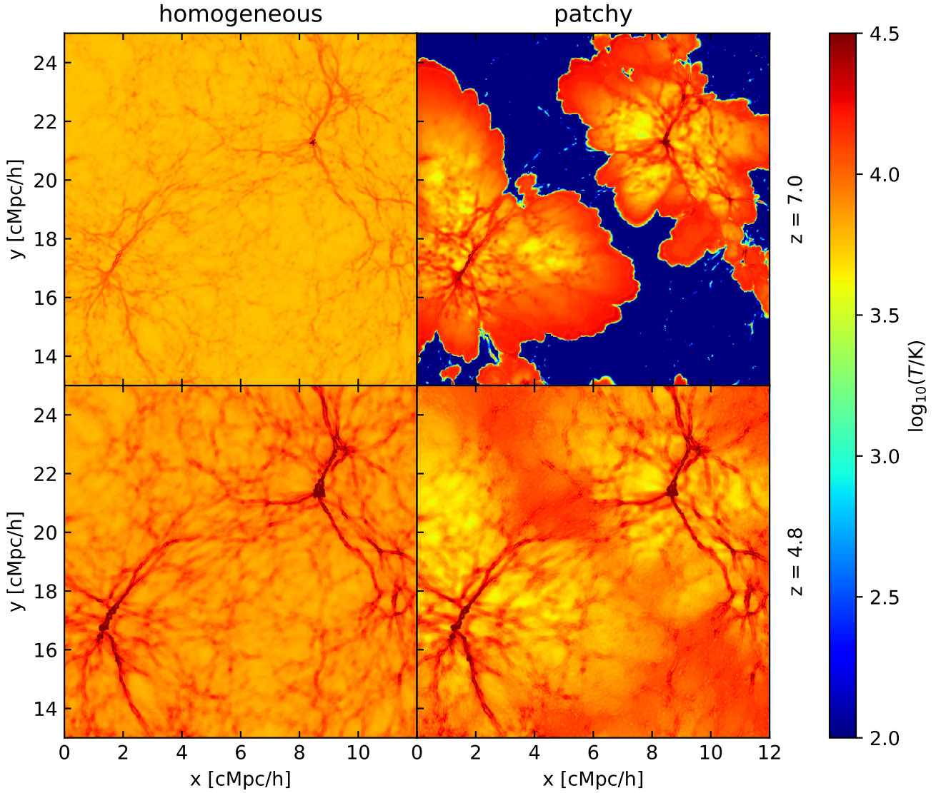
Figure 6. Gas temperature in a thin slice through our matched homogeneous and patchy simulations which complete reionization at z_r = 5.3 . During reionization (redshift 7, both runs \sim 45\% neutral fraction, upper panels) the gas temperature in the simulation with the homogeneous UVB has only small fluctuations which largely trace the gas density, as expected from the narrow density-temperature relation shown in Fig. 5. In contrast the temperature in the patchy simulation differs by orders of magnitude between ionized and neutral regions. Some of the highest temperatures (outside shock heated regions) are found near the ionization fronts in recently ionized gas which had little time to subsequently cool. After reionization (redshift 4.8, lower panels), the temperature in the homogeneous simulation still looks qualitatively similar (except for more pronounced shock heating than at z = 7 ). In the patchy simulation, all of the gas has been photoheated as well, but large scale temperature fluctuations that are relics of the patchy reionization process are still clearly visible. The highest temperatures (except for shock heated gas) are found in regions that have been reionized late.
