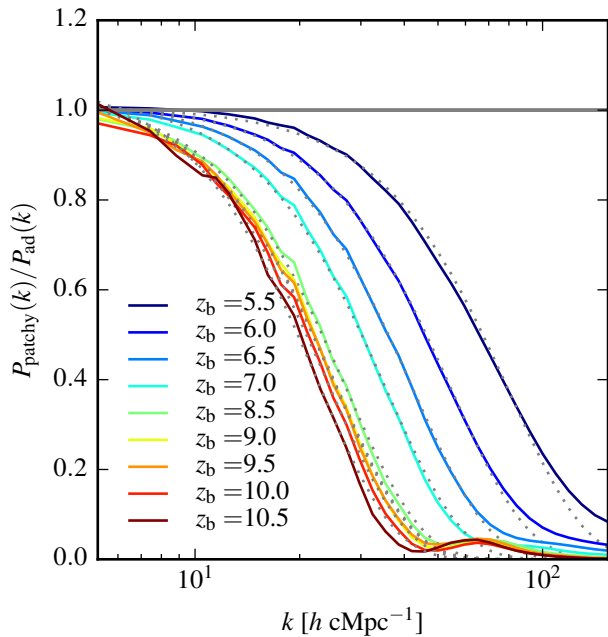
Figure 12. Impact of patchy reionization on small scale structure in the low-density IGM. Shown are ratios of the gas density ( \delta ) power spectra in the z_r = 5.3 patchy and non-radiative (“adiabatic”) simulations. Results are shown at z = 4.8 for regions with different mean reionization redshifts ( z_b in the figure legend denotes the center of the \Delta z = 0.5 bins into which the regions are sorted by their mean local reionization redshift). Regions that have been reionized earlier show a larger suppression of small scale power. All regions included here have a mean gas density of 0.2 < \Delta < 0.4 (in units of the mean cosmic baryon density), corresponding to low-density IGM that the Lyman- \alpha forest is sensitive to. The dotted lines are fits to the solid curves assuming the functional form given in Eq. (2).
