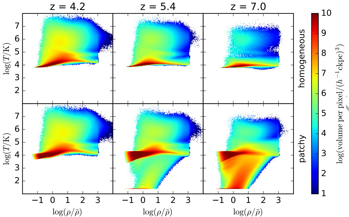
Figure 5. Volume-weighted temperature-density distribution of gas in the patchy simulation that completes reionization at z_r = 5.3 (bottom panels) and in the matched homogeneous simulation (top panels) at redshifts 4.2, 5.4 and 7.0. Both simulations have, by construction, similar volume-weighted neutral fractions of \sim 0\% , 4\% , 45\% at these redshifts, respectively. During reionization, cold gas that has not yet been ionized is present in the patchy run. In contrast, the same gas is partly ionized and heated in the homogeneous simulation. After reionization, the temperature-density relation in the patchy simulations is still broader at low densities.
