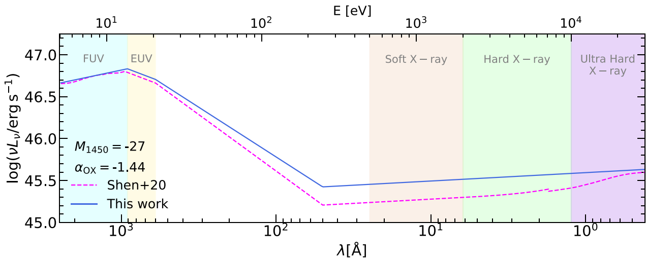
Figure 1. The fiducial power-law quasar SED used in this work (solid blue curve) compared to the SED template from Shen et al. (2020) (dashed fuchsia curve). Both SEDs are normalized at 1450 Å to correspond to an absolute AB magnitude M_{1450} = -27 . The SED is modelled as a broken power law, f_\nu \propto \nu^\alpha , with spectral index \alpha_{\text{FUV}} = -0.61 in the range \lambda = 912\text{--}2500 Å (far UV), \alpha_{\text{EUV}} = -1.70 in the range \lambda = 600\text{--}912 Å (extreme UV), and \alpha_X = -0.9 at \lambda \leq 50 Å (X-ray). The X-ray part of the spectrum is normalized with an optical-to-X-ray spectral index of \alpha_{\text{OX}} = -1.44 . The SED in the range \lambda = 50\text{--}600 Å connects the UV and X-ray sections of the spectrum. The shaded regions indicate common wavelength bands. Our fiducial model corresponds to an ionizing photon emission rate of \dot{N} = 1.64 \times 10^{57} \text{ s}^{-1} .
