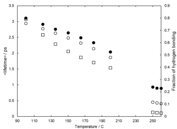
Fig. 2. Average hydrogen bond lifetime (open squares for methanol) and fraction of hydrogen bonding (open circles for methanol; closed circles for ethanol) versus temperature.
