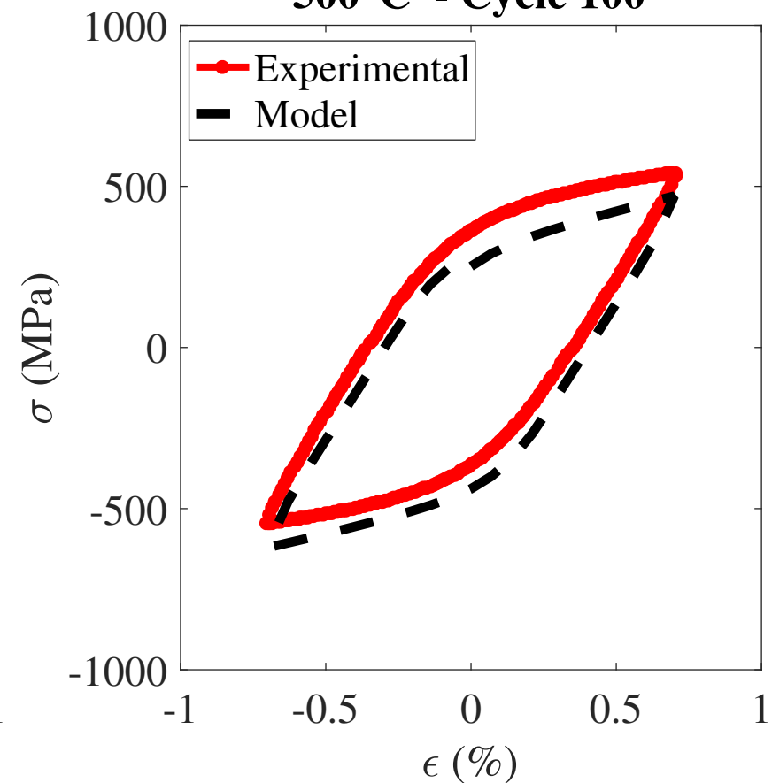
500°C - Cycle 100
