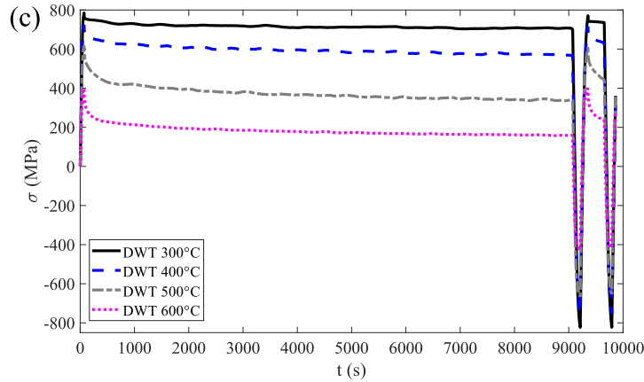
Figure 3: Stress relaxation during 1st and 2nd cycles of the selected dwell-type waveforms.
