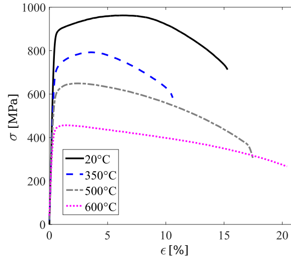
Figure 4: Engineering stress versus engineering strain plots showing the effect of temperature on the tensile properties of the FV566 steel.
