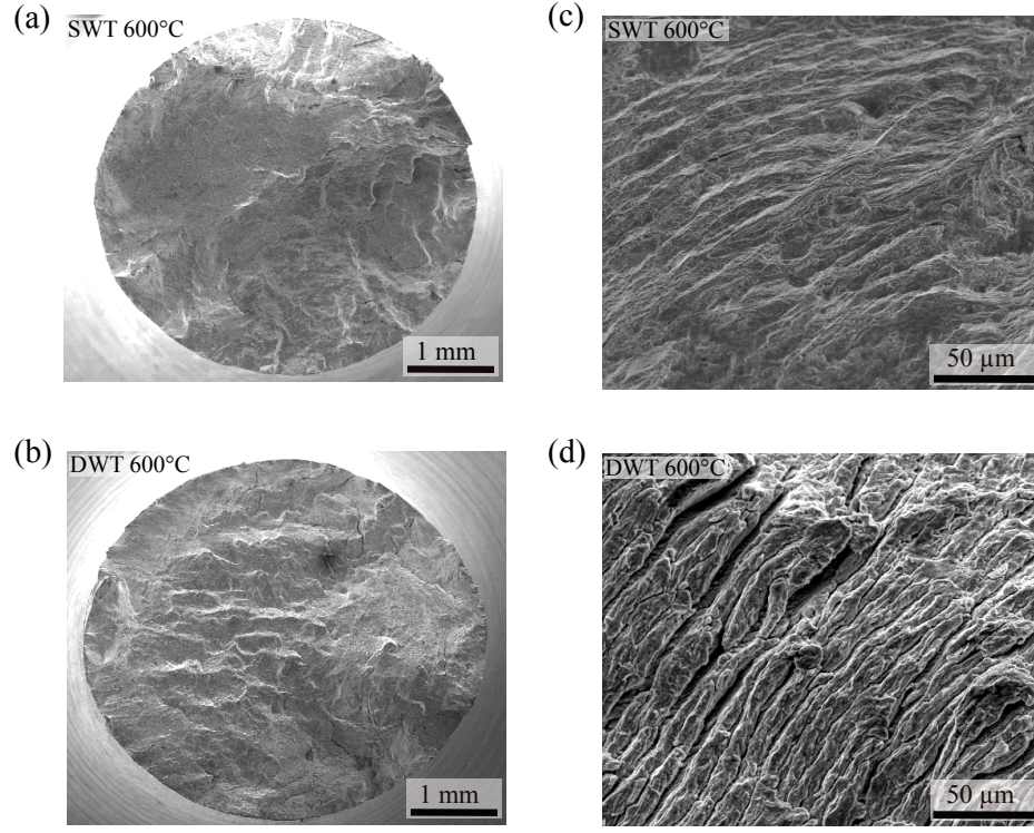
Figure 2: Scanning electron micrographs of the fracture surface features of FV566 steel that was deformed by fatigue loading at temperature of 600 C, showing: (a-b) overall morphology of failure normal to the loading axis and (c-d) high magnification observation of rough fracture surface revealing beachmarks and surface cracks caused during saw-tooth and swell-type loadings respectively.
