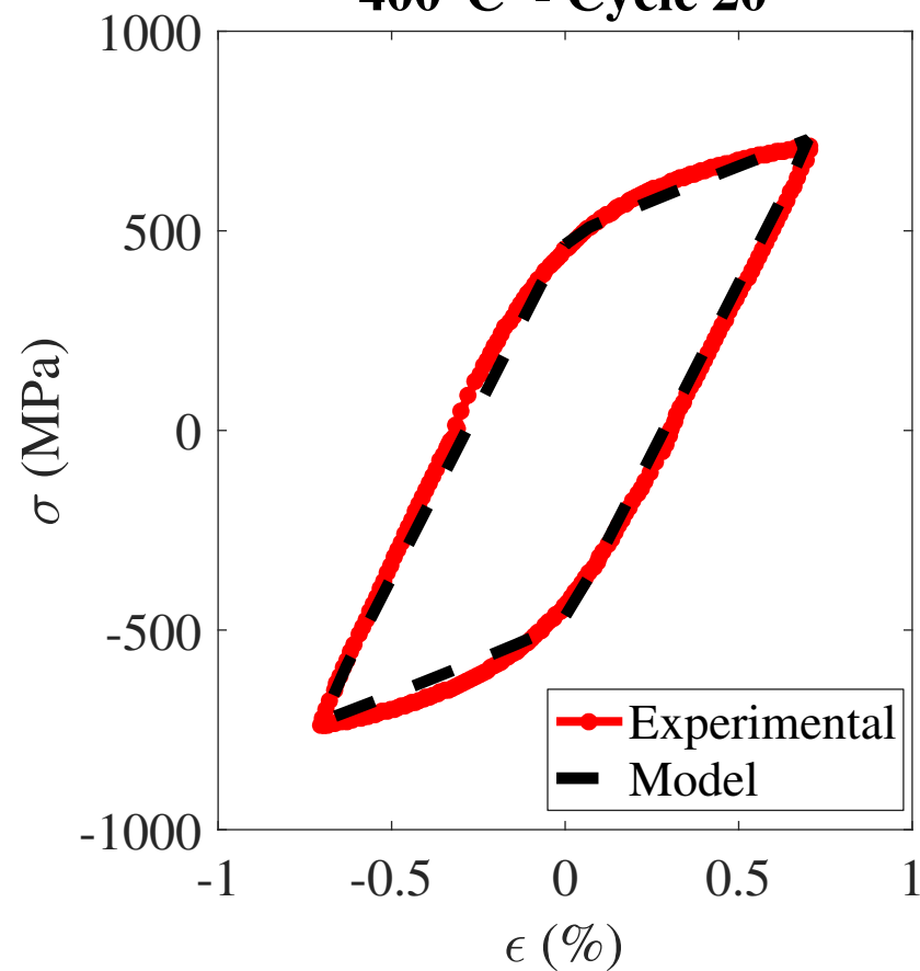
400°C - Cycle 20
