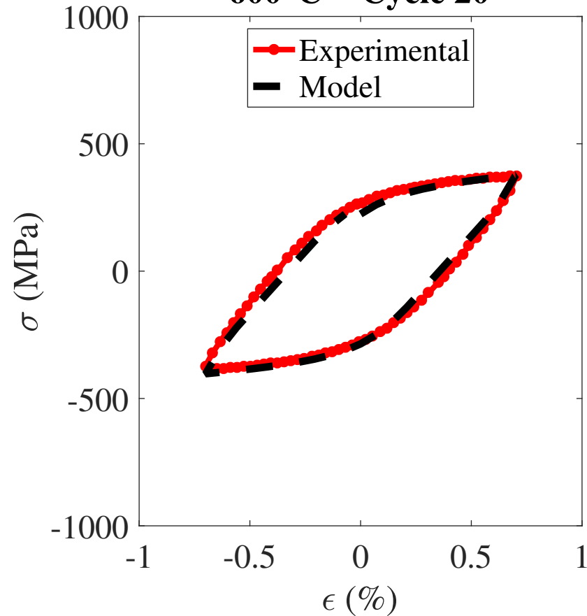
600°C - Cycle 20
