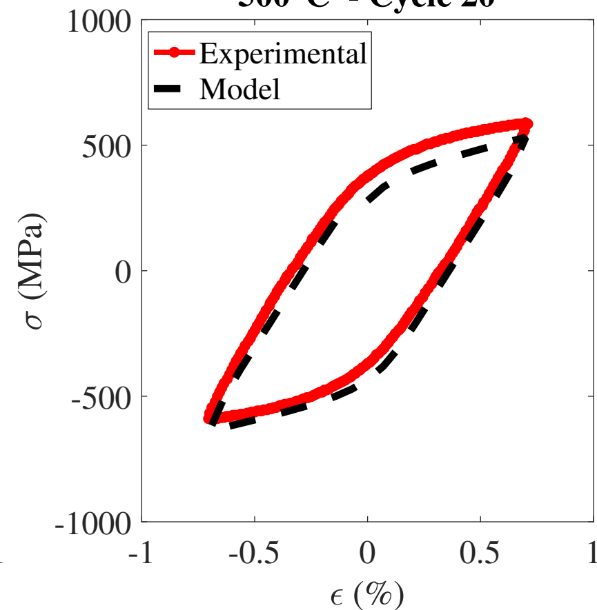
500°C - Cycle 20
