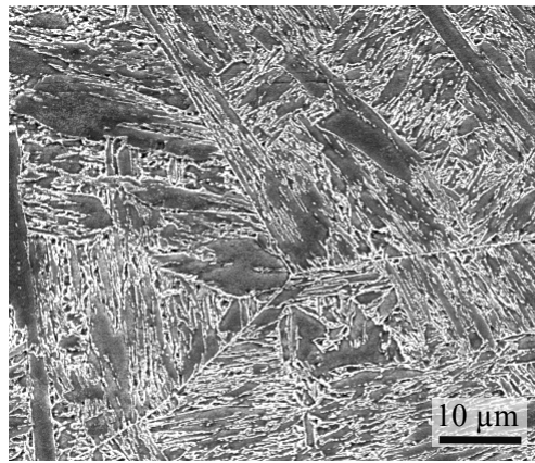
Figure 1: An FEG-SEM image of the chemically etched FV566 material in as received aged state showing typical martensitic microstructure.
