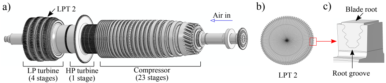
Figure 1: Gas turbine rotor components showing a) compressor, low and high pressure turbine sections, b) 2nd stage of the low pressure turbine, c) a fir-tree joint through which mechanical loads are transferred from the blade to the rotor.
