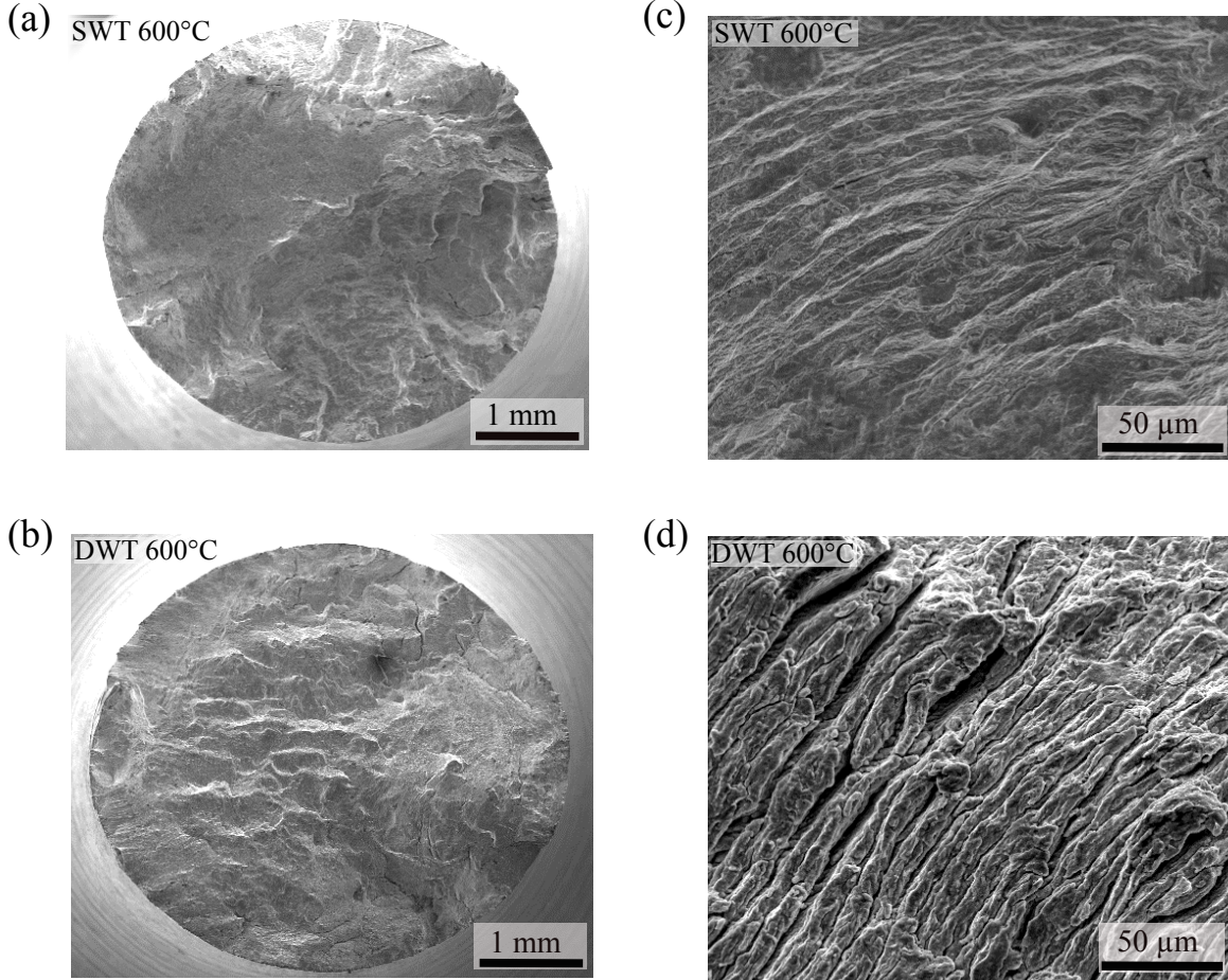
Figure 6: Scanning electron micrographs of the fracture surface features of FV566 steel that was deformed by fatigue loading at temperature of 600°C, showing: (a-b) overall morphology of failure normal to the loading axis and (c-d) high magnification observation of rough fracture surface revealing beachmarks and surface cracks caused during saw-tooth and swell-type loadings respectively.
