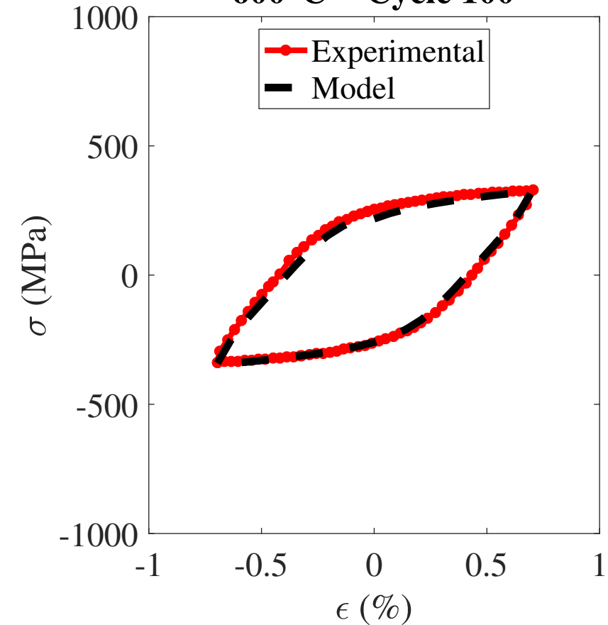
600°C - Cycle 100
