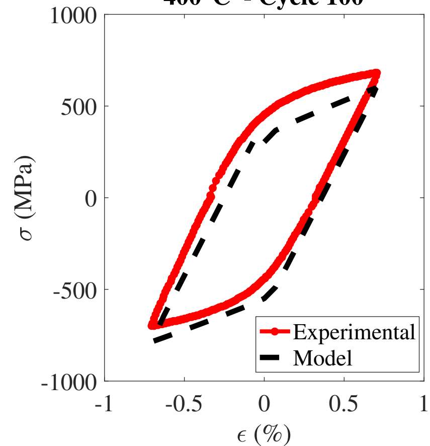
400°C - Cycle 100
