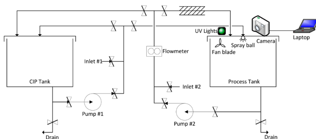
Figure 2. Experimental rig scheme.
