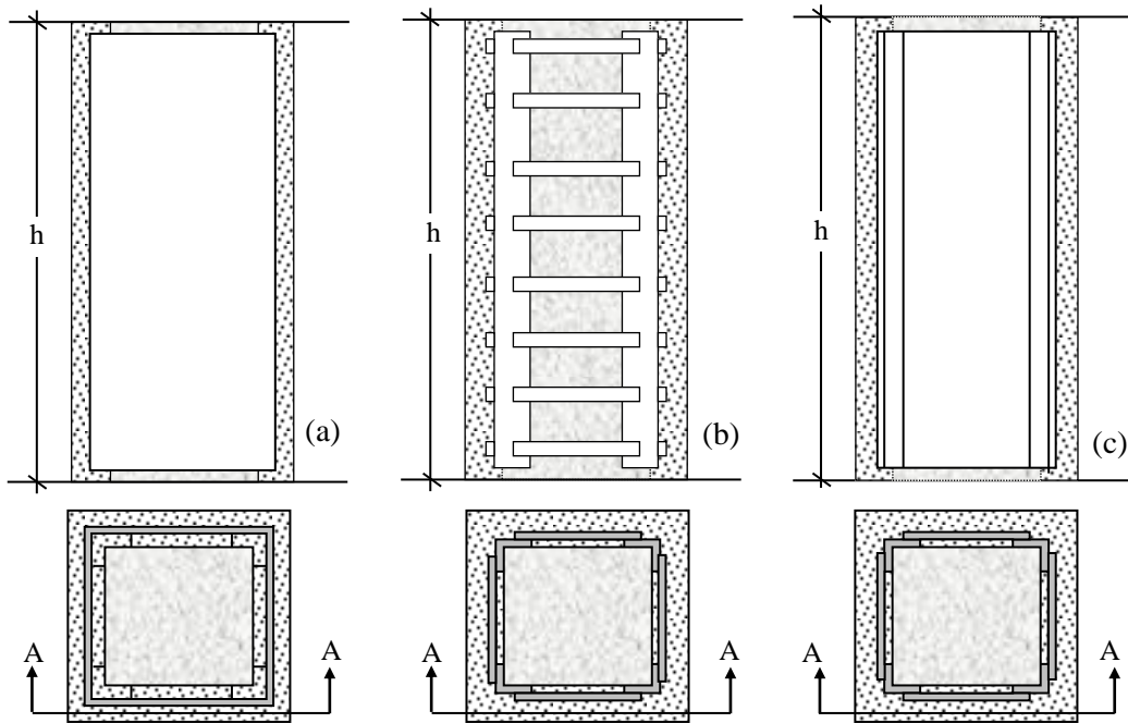
Fig. 2 (a) Steel jacketing; (b) Steel cage technique using steel straps or (c) steel plates
