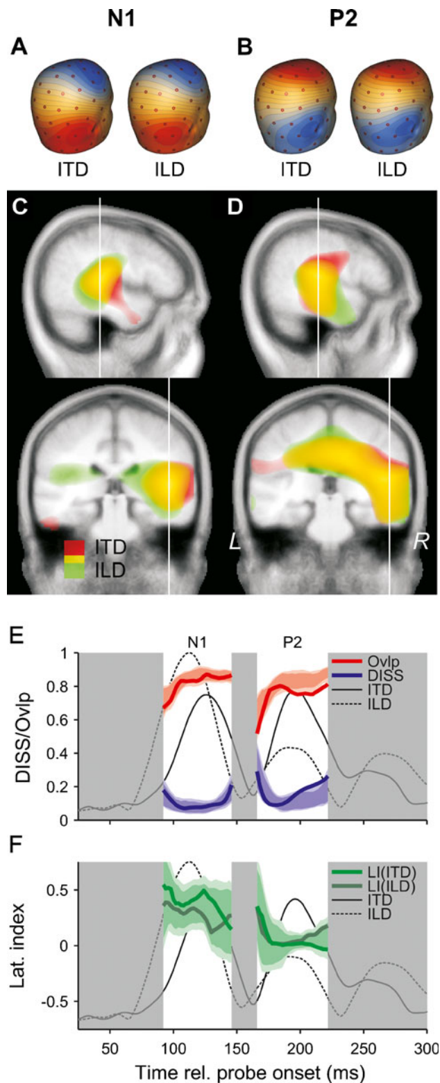
FIG. 5. Comparative source analysis of average ITD- and ILD-only responses. A, B Scalp voltage maps of the N1 ( A ) and P2 ( B ) deflections in the ITD- ( left ) and ILD-only ( right ) responses. The maps were taken from the middle of the rising flank of the respective deflection (106 ms for the N1 and 180 ms for the P2). C, D Distributed source estimates based on the scalp maps shown in A and B , projected onto right sagittal ( top ) and coronal ( bottom ) slices of a Talairach average brain. The source distributions for the ITD and ILD responses are superposed, with the red highlight showing the distribution for the ITD response and the green highlight showing the distribution for the ILD response; the yellow highlight shows where the two distribution overlap. The source distributions for the N1 and P2 are shown in the left and right panels ( C, D ). The thin, white lines show the slice positions. E Global dissimilarity (DISS) between the scalp maps ( bold, blue lines ) and spatial overlap (Ovlp) between the source distributions ( bold, red lines ) of the ITD- and ILD-only responses, calculated within the time ranges of the N1 and P2 ( highlighted by the white background ). The Ovlp was expressed as a proportion of the average total volume of each distribution. The thin, solid and dashed lines show the GFP of the ITD- and ILD-only responses, scaled to the maximum of the ILD-only response. Note that the DISS increases as the response amplitude decreases towards the edges of the N1 and P2 time ranges, because the scalp maps become dominated by noise. The blue- and red-shaded areas represent the null distributions of the DISS and Ovlp, based on 512 permutation samples. The darker shading shows the 5–95, and the lighter shading the 1–99 percentile ranges of the distributions. F Hemispheric lateralization indices (LIs) of the ITD- ( bold, light-green lines ) and ILD-only responses ( bold, dark-green lines ). The green-shaded areas represent the null distributions of the difference between the LIs for the ITD and ILD conditions, shifted to center on the average LI between the ITD and ILD conditions. Again, the darker shading shows the 5–95, and the lighter shading the 1–99 percentile ranges.
