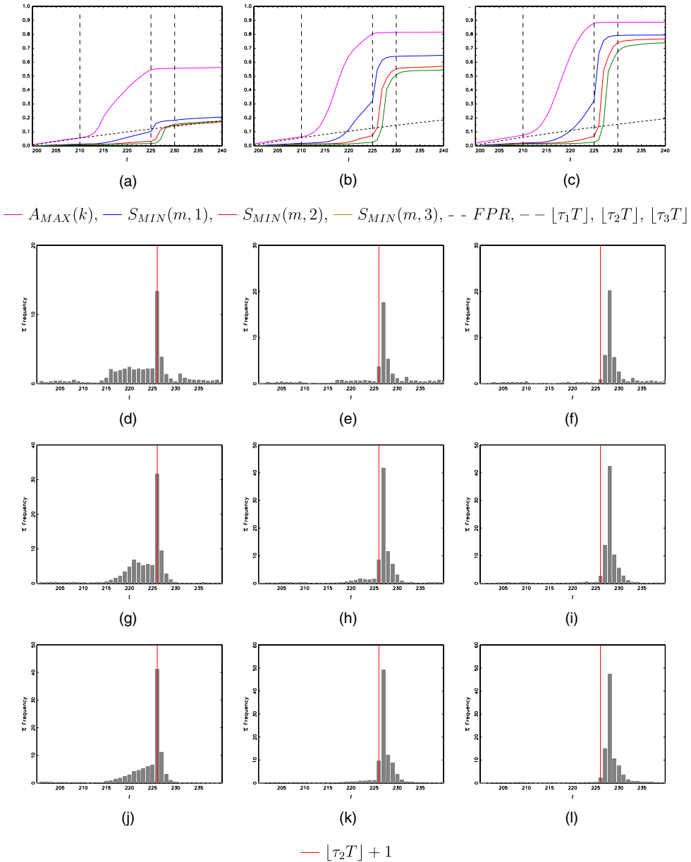
FIGURE 5. Rejection frequencies of A_{MAX}(k) and S_{MIN}(m, n) , and histograms of S_{MIN}(m, n) detection dates: \lceil \tau_1 T \rceil = 210 , \lceil \tau_2 T \rceil = 225 , \lceil \tau_3 T \rceil = 230 , \delta_1 = 0.01 and \delta_2 = 0.005 . (a) m = k = 5 ; (b) m = k = 10 ; (c) m = k = 15 ; (d) S_{MIN}(5, 1) ; (e) S_{MIN}(5, 2) ; (f) S_{MIN}(5, 3) ; (g) S_{MIN}(10, 1) ; (h) S_{MIN}(10, 2) ; (i) S_{MIN}(10, 3) ; (j) S_{MIN}(15, 1) ; (k) S_{MIN}(15, 2) ; (l) S_{MIN}(15, 3)
