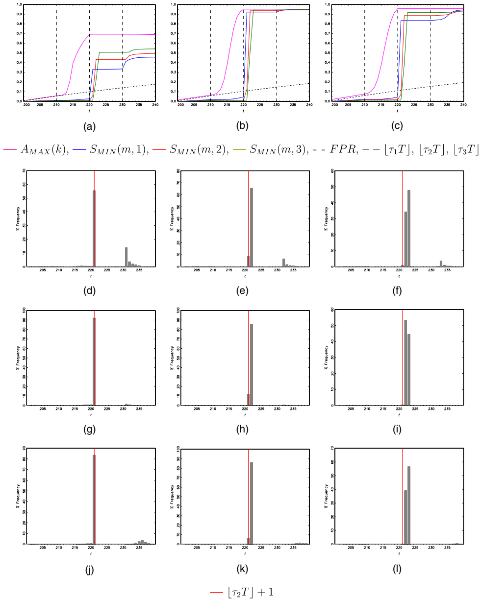
FIGURE 6. Rejection frequencies of A_{MAX}(k) and S_{MIN}(m, n) , and histograms of S_{MIN}(m, n) detection dates: \lfloor \tau_1 T \rfloor = 210 , \lfloor \tau_2 T \rfloor = 220 , \lfloor \tau_3 T \rfloor = 230 , \delta_1 = 0.02 and \delta_2 = 0.03 . (a) m = k = 5 ; (b) m = k = 10 ; (c) m = k = 15 ; (d) S_{MIN}(5, 1) ; (e) S_{MIN}(5, 2) ; (f) S_{MIN}(5, 3) ; (g) S_{MIN}(10, 1) ; (h) S_{MIN}(10, 2) ; (i) S_{MIN}(10, 3) ; (j) S_{MIN}(15, 1) ; (k) S_{MIN}(15, 2) ; (l) S_{MIN}(15, 3)
