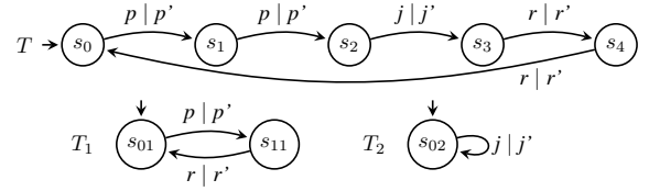
Figure 1: Process recipe T and manufacturing resources T_1 and T_2 . The error states s_{err} for each transducer are not shown
