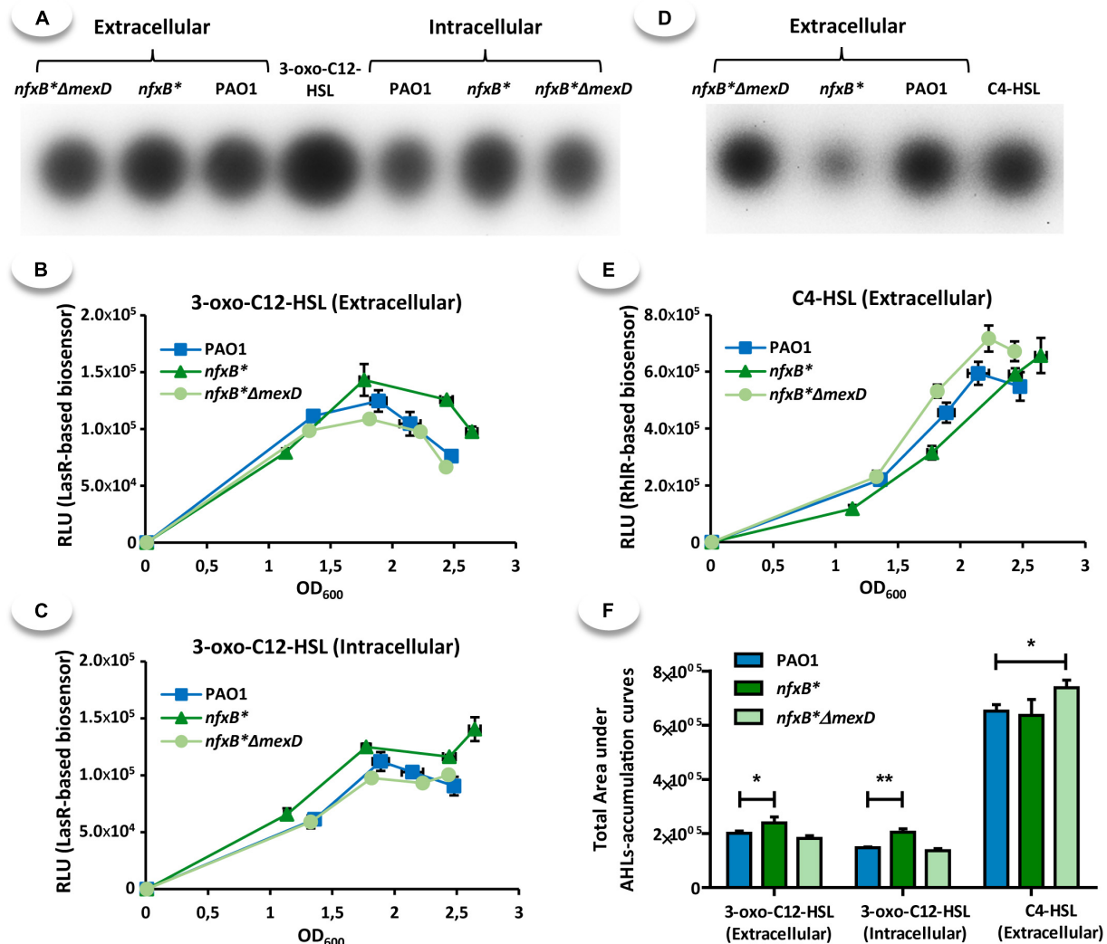
FIGURE 4 | The nfxB* mutant displays minor alterations in the kinetic of accumulation of 3-oxo-C12-HSL autoinducer. TLCs (A,D) and time course accumulation assays (B,C,E) were used to determine the accumulation of either 3-oxo-C12-HSL or C4-HSL autoinducer compounds. The samples for the TLC assays were extracted from cultures in late exponential phase ( OD_{600} = 1.7 ) and the samples for the time course assay were taken at different time along the cell cycle (4, 5, 6, and 7 h post-inoculation). The area under the curve of each time course assay was calculated (F) and statistical significances were evaluated by using a Student's two-tailed test with a confidence interval of 95% (* P < 0.05 ; ** P < 0.01 ; *** P < 0.001 ). As shown, the overexpression of MexCD-OprJ has a slightly but significant effect on 3-oxo-C12-HSL accumulation. The nfxB* strain presented higher levels of 3-oxo-C12-HSL than PAO1 and nfxB* Δ mexD both outside (A,B,F) and inside the cells (A,C,F). In contrast, the supernatant accumulation of C4-HSL in late exponential phase was lower in the MexCD-OprJ overexpressing mutant as compared with PAO1 and nfxB* Δ mexD strains (D,E). However, the quantification of total area under the curves (F) only showed a significant increase in nfxB* Δ mexD strain respect to both PAO1 and nfxB* .
