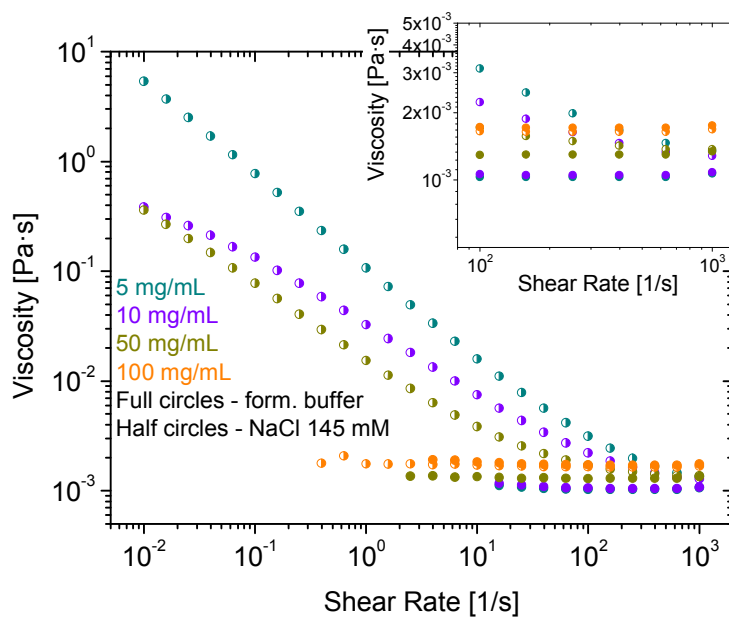
Fig. 5 Viscosity curves for rAlbumin solutions diluted in 145 mM NaCl buffer, in comparison to the material in formulation buffer, at the same concentrations: 5, 10, 50 and 100 mg/mL. Half circles – rAlbumin in 145 mM NaCl only; full circles - rAlbumin in formulation buffer. Inset focuses on the viscosities of these samples at the higher shear rates.
