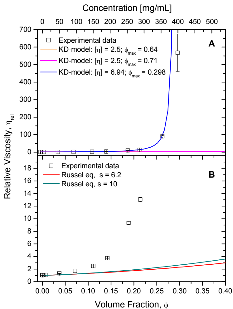
Fig. 7 A Experimental cone-and-plate rheometry data (squares) plotted against expected data (lines) from Krieger-Dougherty's equation (eq. 3) with fixed parameters. Relative viscosity was calculated by dividing each sample's ( \eta (1000 s -1 )) by the buffer's viscosity ( \eta_0 = 1.038 \pm 0.013 mPa.s). For both lines, [\eta] was fixed to 2.5, but different \phi_{max} were used: 0.64 (orange); 0.71 (magenta). See text for more details. Data was fitted to Krieger-Dougherty's equation using free parameters (blue). Computed parameters were [\eta] = 6.9 \pm 0.14 , \phi_{max} = 0.30 \pm 0.0025 , with r^2 = 0.999 and \chi^2 = 0.26 . Experimental data used for was up to 350 mg/mL. B Experimental cone-and-plate rheometry data (squares) plotted against expected data (lines) from Russel's equation (eq. 4) using fixed parameters. For both lines, [\eta] was fixed to 2.5, but s was: 6.2 (red line); 10 (green line).
