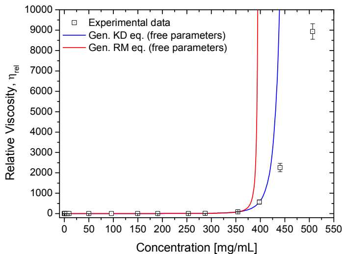
Fig. 8 Experimental data fitted to the generalised Krieger-Dougherty equation (eq. 8; blue line). Fitting parameters were [\eta]_w = 0.00517 \pm 1.1 \times 10^{-4} mL/mg, w^* = 399 \pm 3.4 mg/mL, with r^2 = 0.999 and \chi^2 = 0.26 . Data used was up to 350 mg/mL. Experimental data fitted to the generalised Ross-Minton equation (eq. 7, red line). Fitting parameters were [\eta]_w = 0.00479 \pm 4.0 \times 10^{-5} mL/mg, w^* = 569 \pm 2.2 mg/mL, with r^2 = 1.0 and \chi^2 = 0.91 . Data used was up to 400 mg/mL. For both plots, relative viscosity was calculated by dividing the sample's \eta(1000s^{-1}) by the buffer's viscosity ( 1.038 \pm 0.013 mPa.s).
