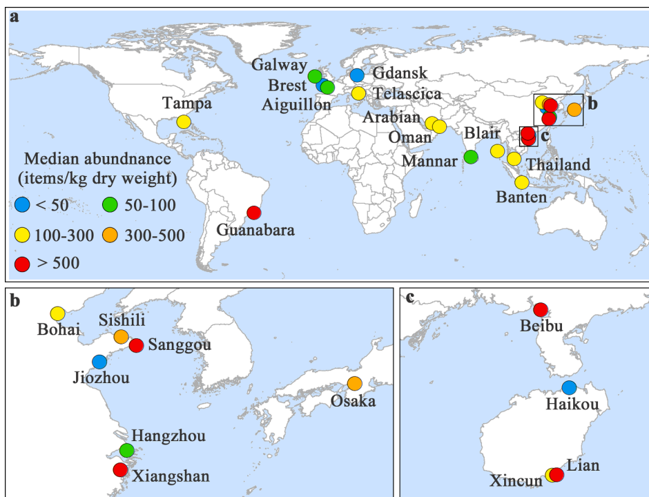
Fig. 2. Geographical distribution of microplastic abundance (a). More detailed views in selected regions (b-c).
