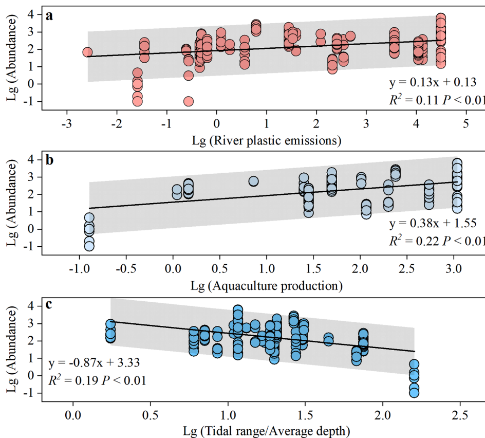
Fig. 3. The effects of river plastic emissions (a), aquaculture production (b) and ratio of tidal range to average water depth (c) on microplastic abundance. The shaded area denotes 95% prediction intervals.
