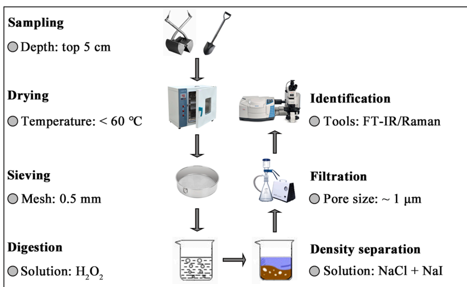
Fig. 8. Suggested sampling and analysis methods for sedimental microplastics.
