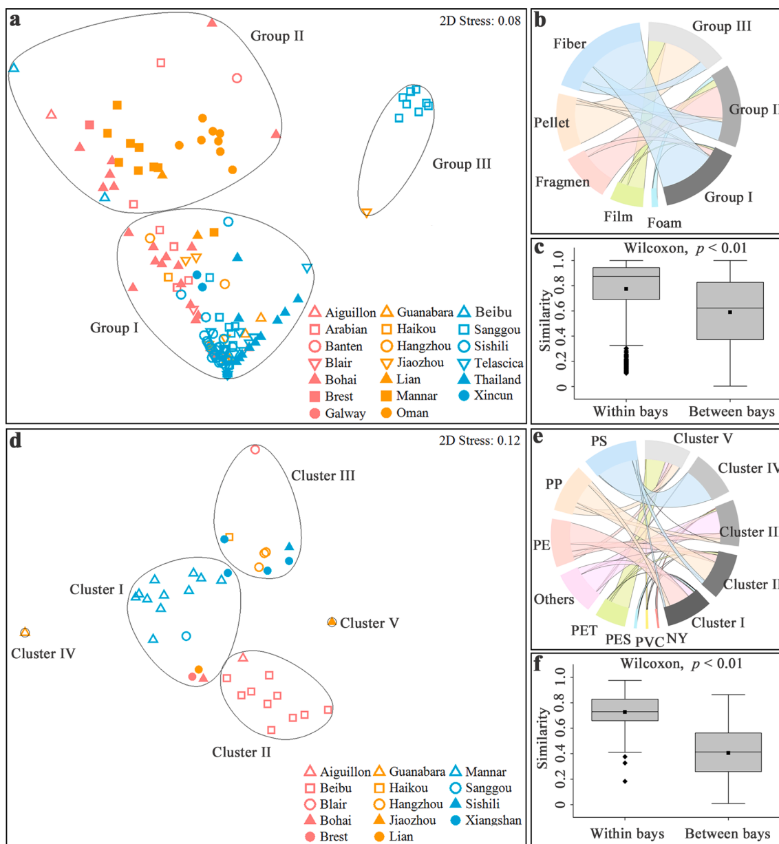
Fig. 6. Similarity in the shape (a-c) and polymer (d-f) composition of microplastics. Classification of samples via Nonmetric Multidimensional Scaling (a, d); Morphological composition of each group (b, e); Similarity coefficients between samples within and between bays (c, f); PS, PP, PE, PET, PES, PVC and NY refer to Polystyrene, Polypropylene, Polyethylene, Polyethylene terephthalate, Polyester, Polyvinylchloride and Nylon, respectively.
