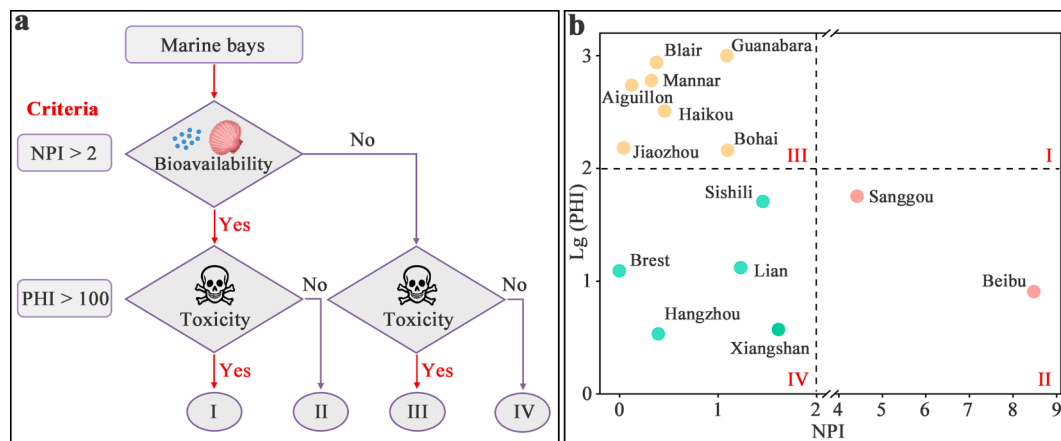
Fig. 7. Environmental risk of microplastics. Risk assessment system (a); Risk ranks of marine bays. NPI and PHI refer to Nemerow pollution index and Polymer hazard index of microplastics, respectively.
