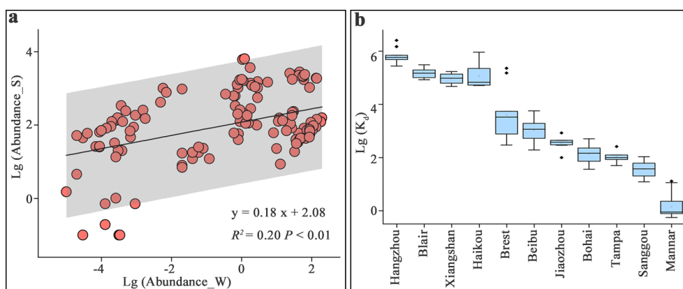
Fig. 5. Relationship between microplastic abundance in water and sediment (a); Sediment-water partitioning coefficients ( K_d ) of microplastics in marine bays (b). Abundance_W and abundance_S refer to microplastic abundance in water and sediment, respectively.
