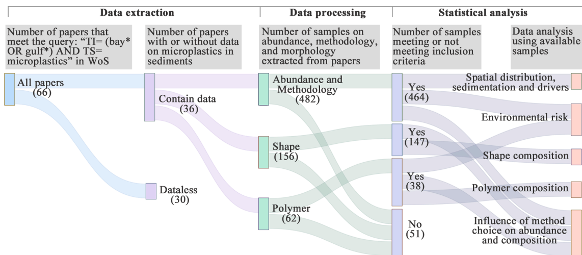
Fig. 1. Framework for data extraction, data processing and statistical analysis of microplastics in the sediment of marine bays. TI, TS and WoS refer to title, topic and Web of Science, respectively.
