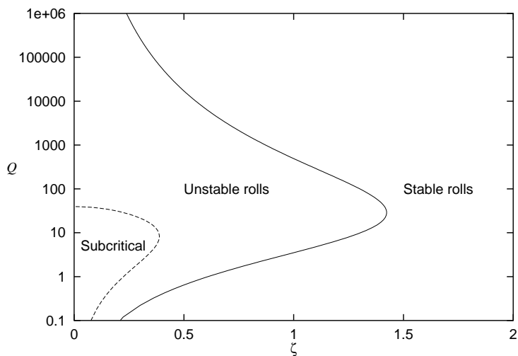
Figure 15. Region of stability of convection rolls in magnetoconvection. To the right of the solid line, rolls are stable. To the left of the dashed line the bifurcation is subcritical. Between the two lines, all rolls are unstable.
