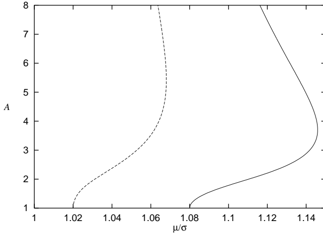
Figure 3. The bifurcation diagram for (3.21)–(3.22) with periodic boundary conditions with L = 5\pi (solid line) and L = 10\pi (dashed line). Solutions take the form (3.27). The vertical axis shows the maximum value of A .
