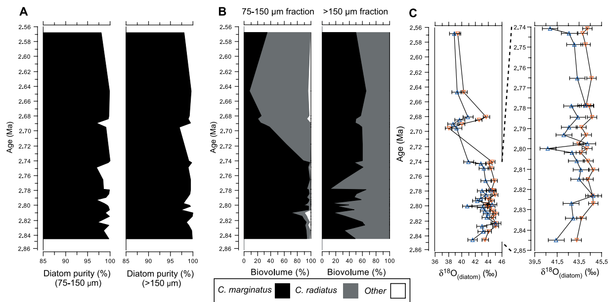
Figure 3. (a) Sample purity, percentage of diatom material relative to all other material. (b) Relative diatom species biovolume in purified samples analyzed for \delta^{18}\text{O}_{\text{diatom}} . (c) Comparison of \delta^{18}\text{O}_{\text{diatom}} measurements from the 75–150 \mu\text{m} fraction (red down triangle) and >150 \mu\text{m} fraction (blue up triangle) between 2.86 Ma and 2.56 Ma. Error bars represent mean, 1\sigma , analytical reproducibility of 0.44‰ in the 75–150 \mu\text{m} fraction and 0.71‰ in the >150 \mu\text{m} fraction.
