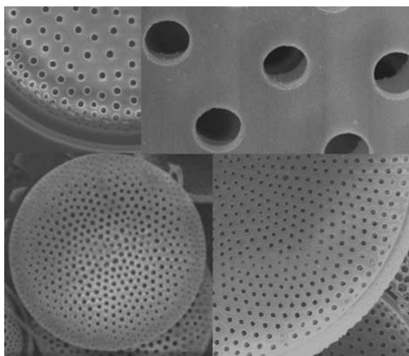
Figure 2. SEM images of diatoms analyzed for \delta^{18}\text{O} from ODP site 882.
