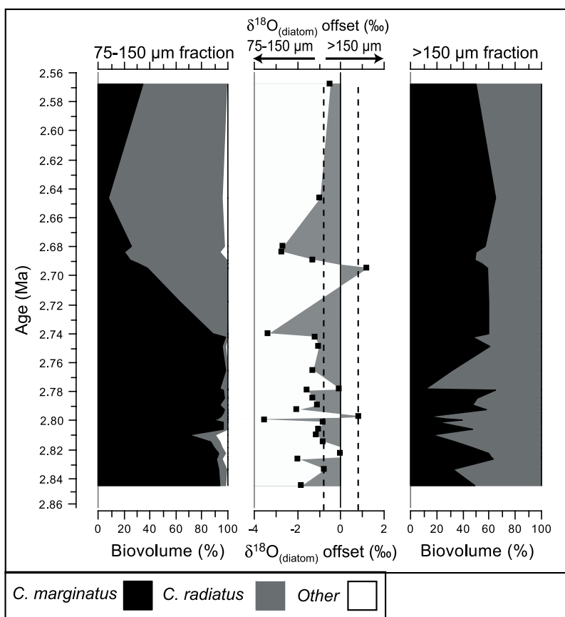
Figure 4. Relative diatom species biovolume in purified samples analyzed for \delta^{18}\text{O}_{\text{diatom}} alongside the magnitude and direction of the \delta^{18}\text{O}_{\text{diatom}} offsets ( >150\ \mu\text{m} fraction minus 75\text{--}150\ \mu\text{m} fraction) between the two size fractions (dashed lines represent the combined analytical reproducibility of 0.84\text{‰} for the two size fractions).
