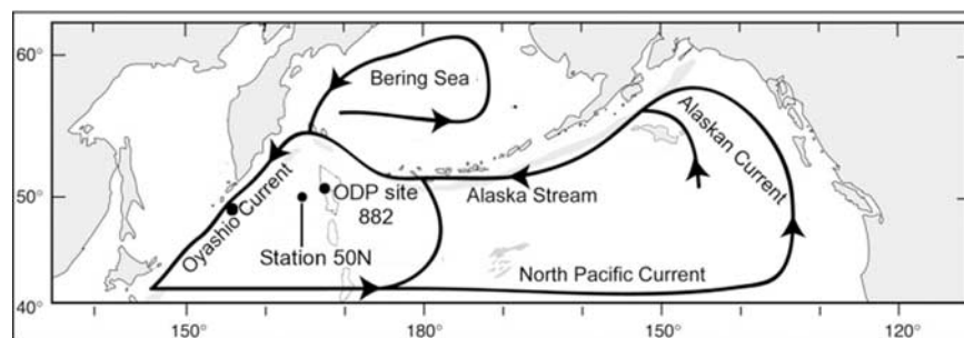
Figure 1. Location of ODP site 882 (50°22′N, 167°36′E) northwest Pacific Ocean together with diatom monitoring station 50N (50.01°N, 165.01°E) and major ocean surface currents in the North Pacific Ocean.
