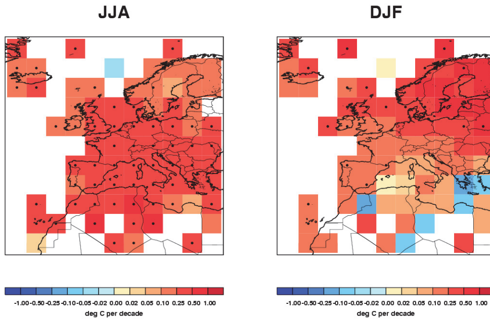
Figure 2. Decadal trends in seasonally averaged temperatures for France and the surrounding regions over the period 1960 to 2010. Monthly mean anomalies from CRUTEM3 (Brohan et al., 2006) are averaged over each 3 month season (June-July-August – JJA and December-January-February – DJF). Trends are fitted using the median of pairwise slopes method (Sen, 1968; Lanzante, 1996). There is high confidence in the trends shown if the 5 th to 95 th percentiles of the pairwise slopes do not encompass zero because here the trend is considered to be significantly different from a zero trend (no change). This is shown by a black dot in the centre of the respective grid box.
