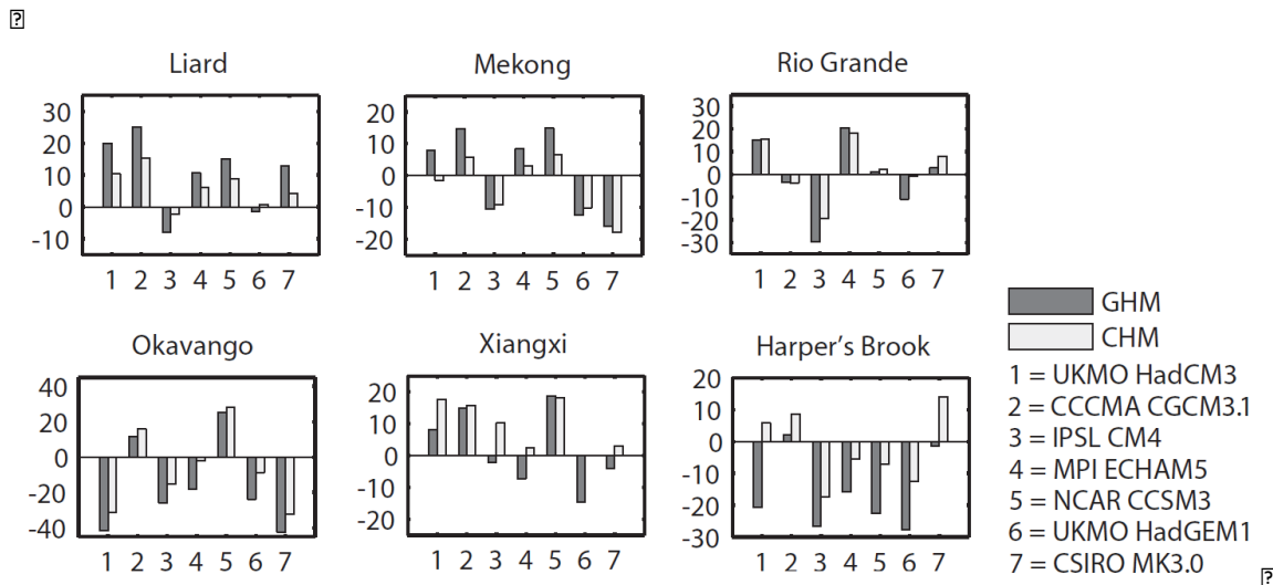
Figure 1. Change in average annual runoff relative to present (vertical axis; %), when a global hydrological model (GHM) and a catchment-scale hydrological model (CHM) are driven with climate change projections from 7 GCMs (horizontal axis), under a 2°C prescribed global-mean warming scenario, for six river catchments. The figure is from Gosling et al. (2011).
