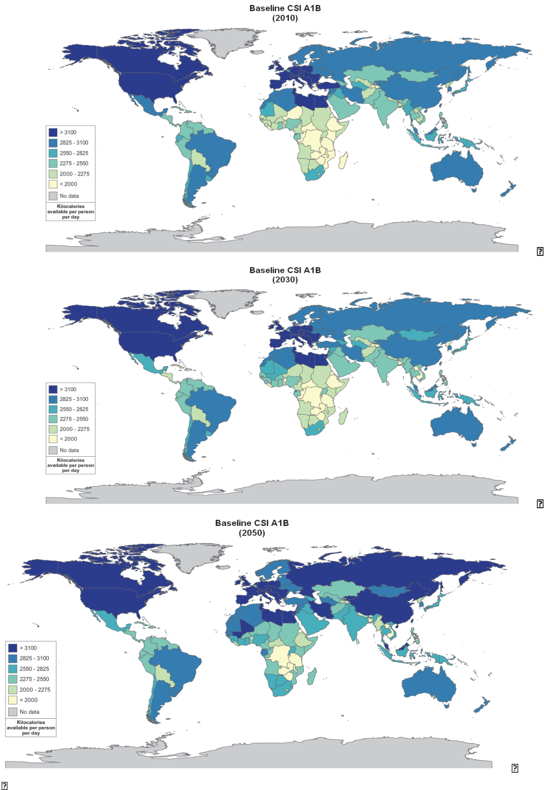
Figure 7. Average daily kilocalorie availability simulated by the CSIRO GCM (CSI) under an A1B emissions scenario and the baseline socioeconomic scenario, for 2010 (top panel), 2030 (middle panel) and 2050 (bottom panel). The figure is from IFPRI (IFPRI, 2010). The changes show the combination of both climate change and socio-economic changes.
