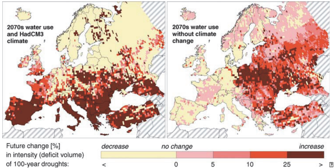
Figure 15. Change in intensity of 100-year droughts, based on comparison between today's climate and water use (1961–1990) and simulations for the 2070s (left map: HadCM3 GCM; right map: only water use scenario, no climate change), under a 1%/year CO 2 increase emissions scenario.
