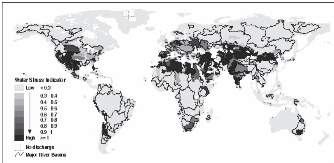
Figure 11. A map of the major river basins across the globe and the water stress indicator (WSI) for the 1961-1990 time horizon. The figure is from Smakhtin et al.
