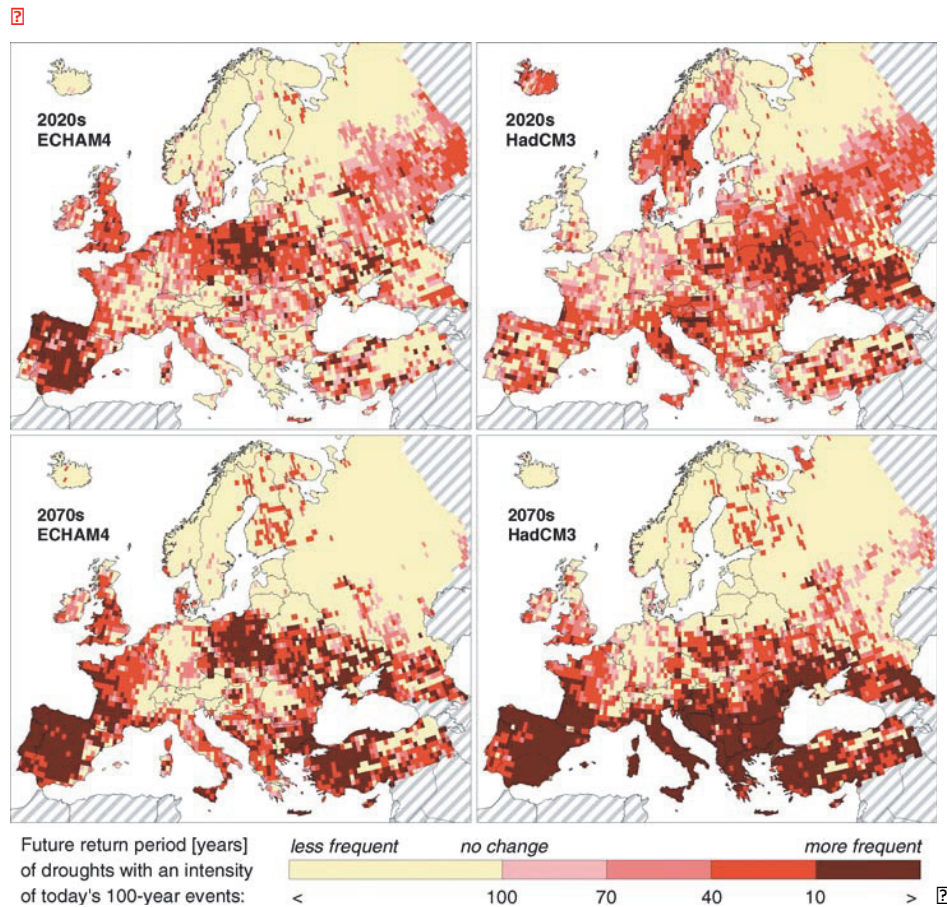
Figure 14. Change in recurrence of 100-year droughts, based on comparisons between today's climate and water use (1961–1990) and simulations for the 2020s and 2070s (ECHAM4 and HadCM3 GCMs), under a 1%/year CO 2 increase emissions scenario. The figure is from Lehner et al. (2006).
