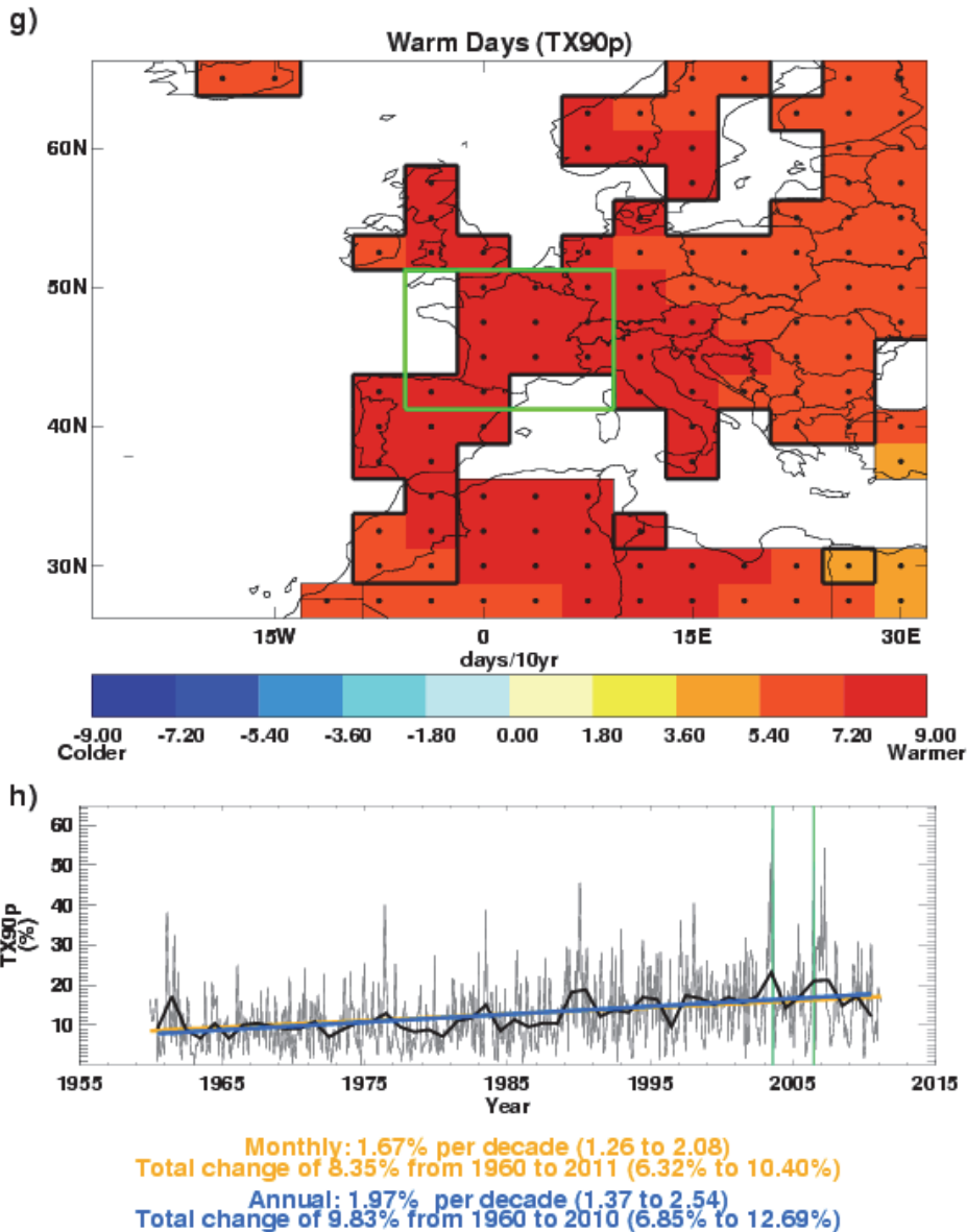
Figure 3. Change in cool nights (a,b), warm nights (c,d), cool days (e,f) and warm days (g,h) for France over the period 1960 to 2010 relative to 1961-1990 from the ECA&D dataset (Klein Tank et al., 2002). a,c,e,g) Grid-box decadal trends. Grid-boxes outlined in solid black contain at least 3 stations and so are likely to be more representative of the wider grid-box. Trends are fitted using the median of pairwise slopes method (Sen, 1968; Lanzante, 1996). Higher confidence in a long-term trend is shown by a black dot if the 5th to 95th percentile slopes are of the same sign. Differences in spatial coverage occur because each index has its own decorrelation length scale (see methodology section); b,d,f,h) Area averaged annual time series for 5.625° W to 9.375° E and 41.25° to 56.25° N as shown by the green box on the map and red box in Figure 1. Thin and thick black lines show the monthly and annual variation respectively. Monthly (orange) and annual (blue) trends are fitted as described above. The decadal trend and its 5th to 95th percentile confidence intervals are stated along with the change over the period for which there are data available. All the trends have higher confidence that they are different from zero as their 5th to 95th percentile slopes are of the same sign. The green vertical lines show the locations of the heat waves in 2003 and 2006.
