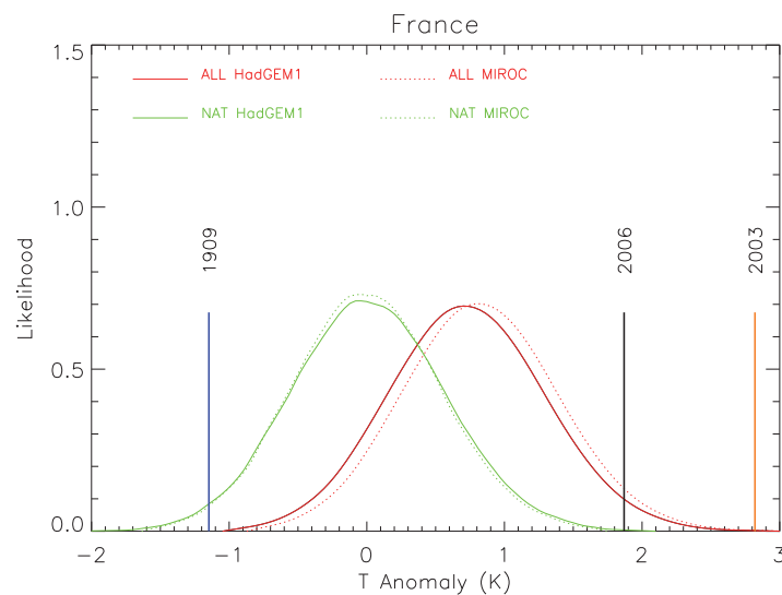
Figure 4. Distributions of the June-July-August mean temperature anomalies (relative to 1961-1990) averaged over a Northern European region that encompasses France (10W-20E, 40-60N – as shown in Figure 1) including (red lines) and excluding (green lines) the influence of anthropogenic forcings. The distributions describe the seasonal mean temperatures expected in recent years (2000-2009) and are based on analyses with the HadGEM1 (solid lines) and MIROC (dotted lines) models. The vertical black line marks the observed anomaly in 2006 and the vertical orange and blue lines correspond to the maximum and minimum anomaly in the CRUTEM3 dataset since 1900 respectively.
